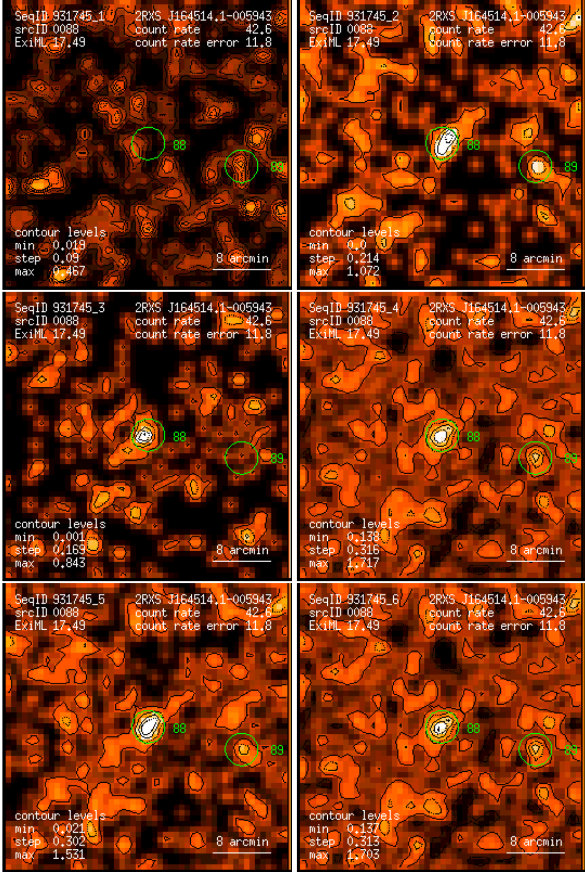
Figure 88: RASS 931745: detection 0088: band rate images, Gaussian filter: (1) PSPC channels 11 – 41, (2) 52 – 90, (3) 91 – 201, (4) 11 – 235, (5) 52 – 201, (6) 11 – 201. Broad band rates in counts/ks. Band rate contour levels in counts/ks/arcmin 2 .
