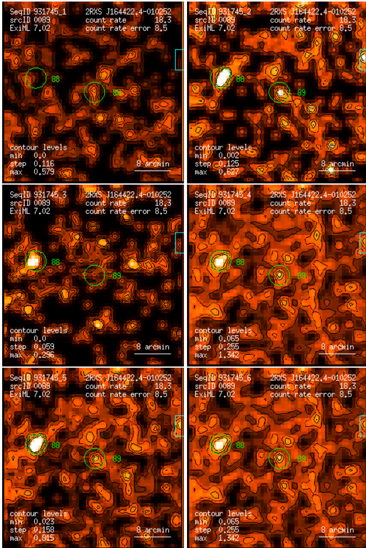
Figure 89: RASS 931745: detection 0089: band rate images, Gaussian filter: (1) PSPC channels 11 – 41, (2) 52 – 90, (3) 91 – 201, (4) 11 – 235, (5) 52 – 201, (6) 11 – 201. Broad band rates in counts/ks. Band rate contour levels in counts/ks/arcmin 2 .
