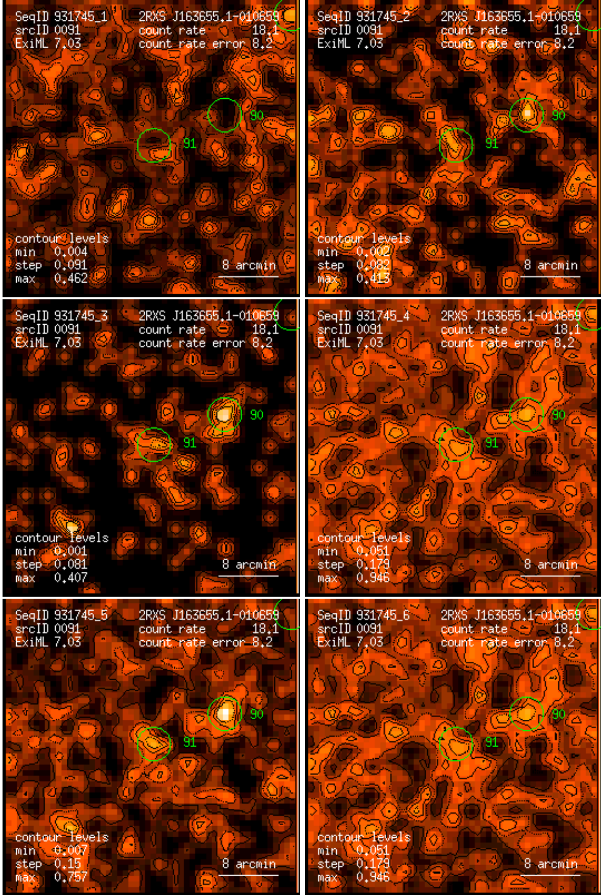
Figure 91: RASS 931745: detection 0091: band rate images, Gaussian filter: (1) PSPC channels 11 – 41, (2) 52 – 90, (3) 91 – 201, (4) 11 – 235, (5) 52 – 201, (6) 11 – 201. Broad band rates in counts/ks. Band rate contour levels in counts/ks/arcmin 2 .
