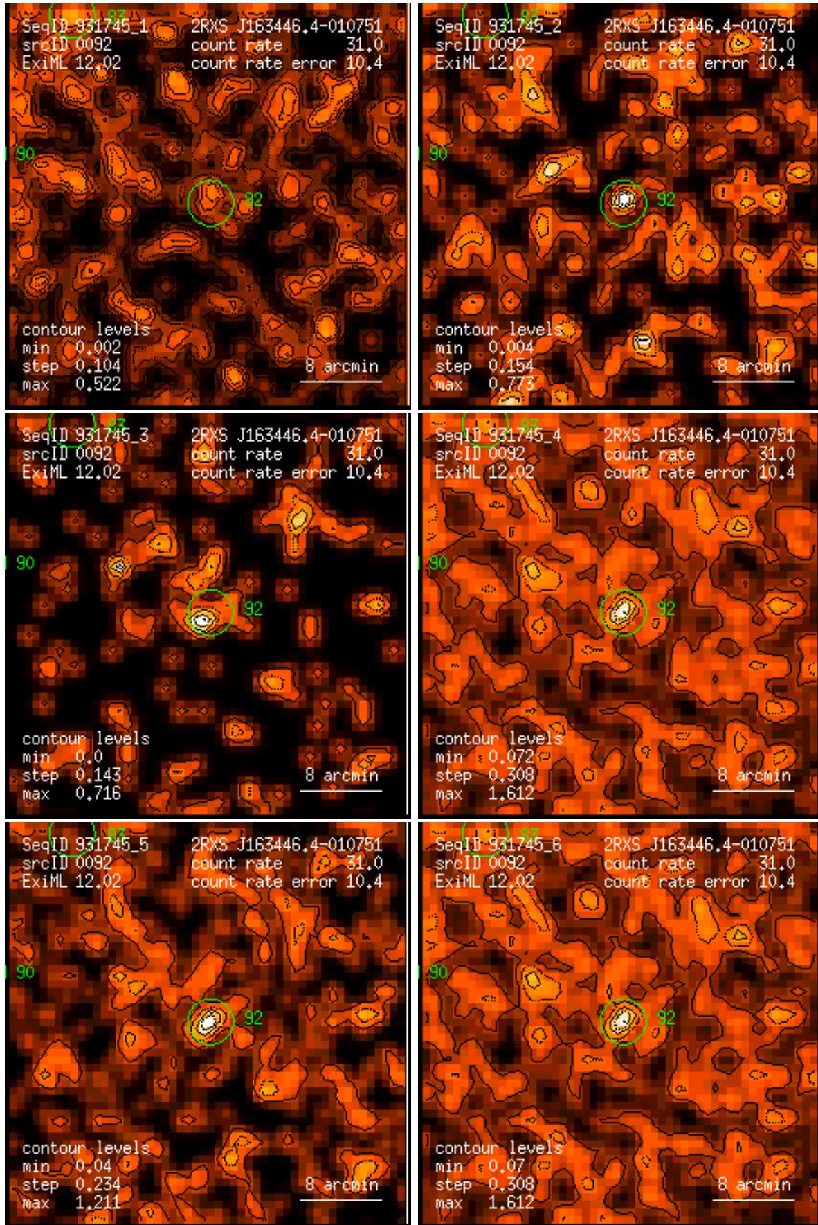
Figure 92: RASS 931745: detection 0092: band rate images, Gaussian filter: (1) PSPC channels 11 – 41, (2) 52 – 90, (3) 91 – 201, (4) 11 – 235, (5) 52 – 201, (6) 11 – 201. Broad band rates in counts/ks. Band rate contour levels in counts/ks/arcmin 2 .
