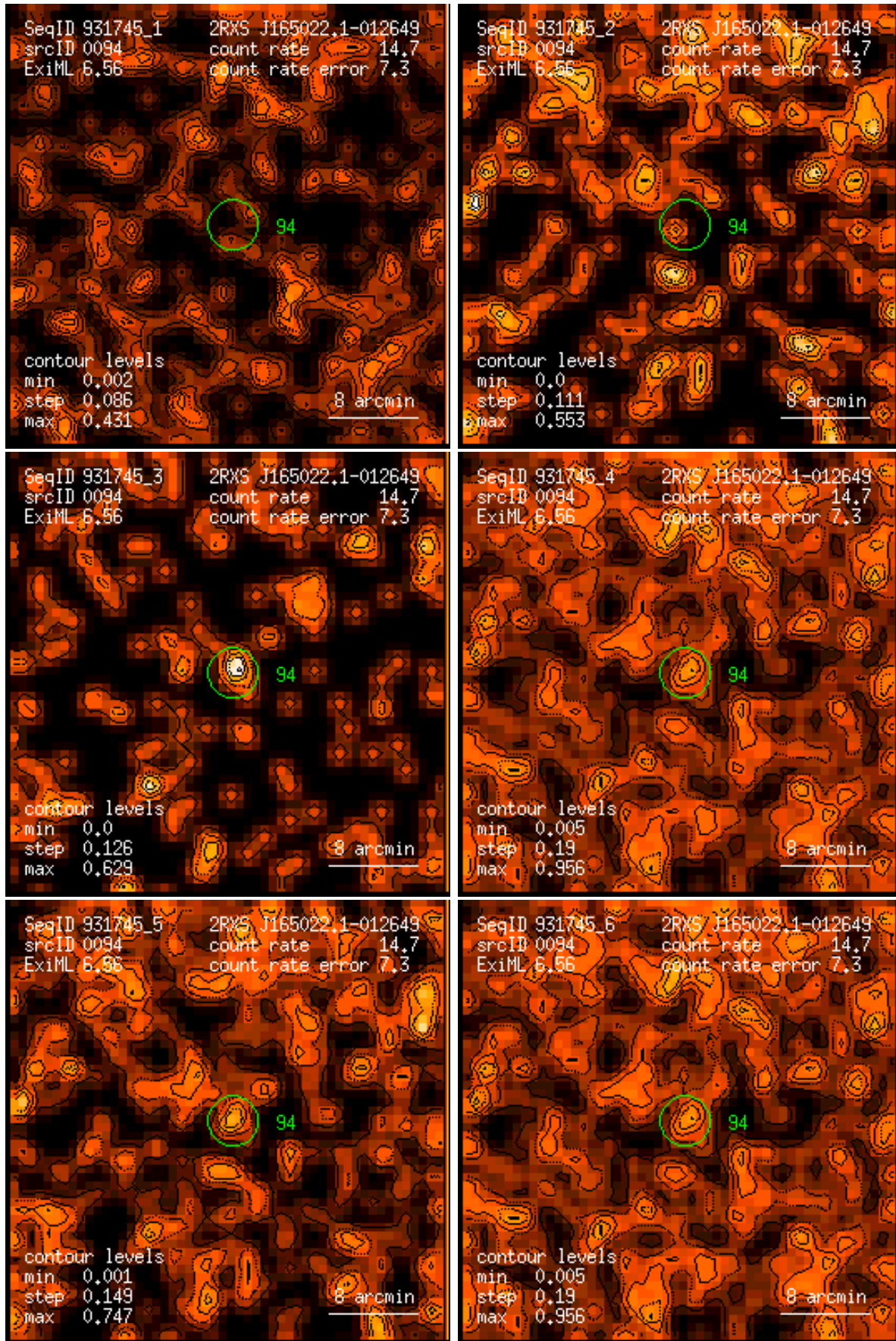
Figure 94: RASS 931745: detection 0094: band rate images, Gaussian filter: (1) PSPC channels 11 – 41, (2) 52 – 90, (3) 91 – 201, (4) 11 – 235, (5) 52 – 201, (6) 11 – 201. Broad band rates in counts/ks. Band rate contour levels in counts/ks/arcmin 2 .
