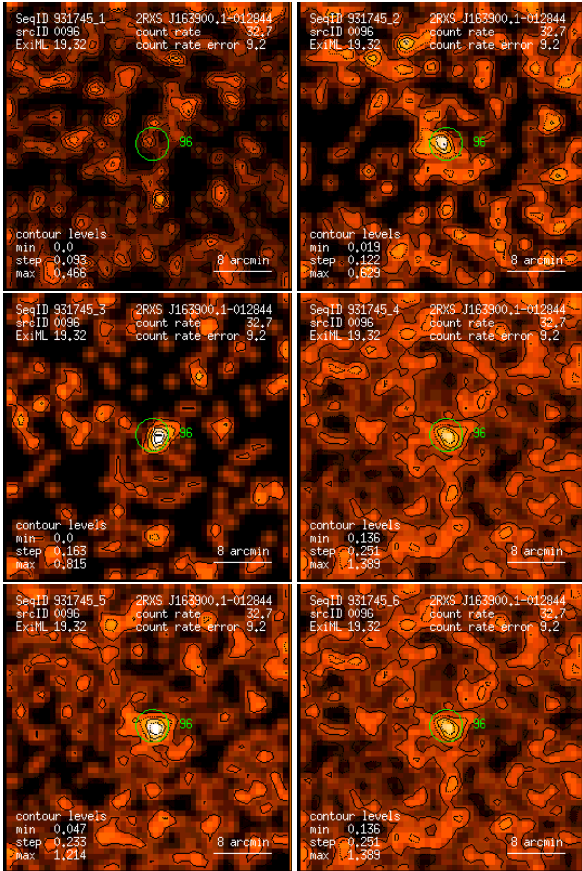
Figure 96: RASS 931745: detection 0096: band rate images, Gaussian filter: (1) PSPC channels 11 – 41, (2) 52 – 90, (3) 91 – 201, (4) 11 – 235, (5) 52 – 201, (6) 11 – 201. Broad band rates in counts/ks. Band rate contour levels in counts/ks/arcmin 2 .
