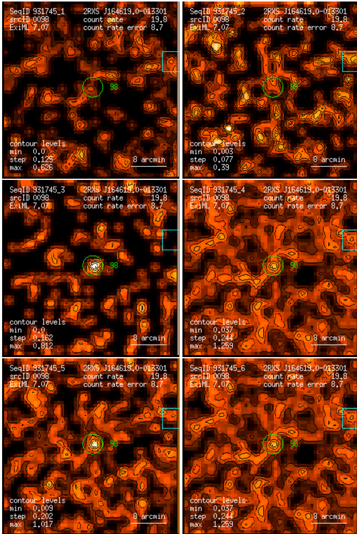
Figure 98: RASS 931745: detection 0098: band rate images, Gaussian filter: (1) PSPC channels 11 – 41, (2) 52 – 90, (3) 91 – 201, (4) 11 – 235, (5) 52 – 201, (6) 11 – 201. Broad band rates in counts/ks. Band rate contour levels in counts/ks/arcmin 2 .
