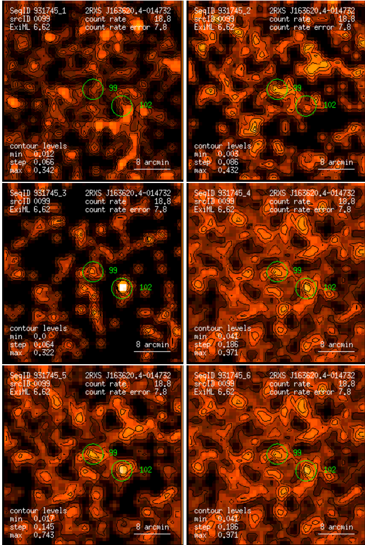
Figure 99: RASS 931745: detection 0099: band rate images, Gaussian filter: (1) PSPC channels 11 – 41, (2) 52 – 90, (3) 91 – 201, (4) 11 – 235, (5) 52 – 201, (6) 11 – 201. Broad band rates in counts/ks. Band rate contour levels in counts/ks/arcmin 2 .
