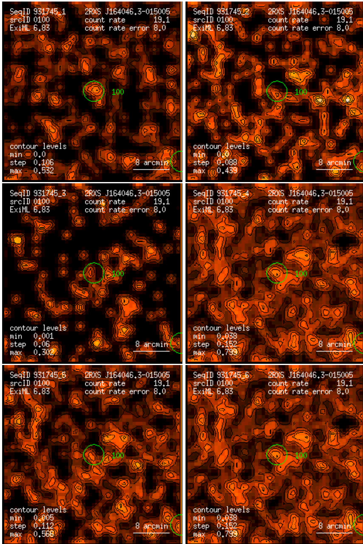
Figure 100: RASS 931745: detection 0100: band rate images, Gaussian filter: (1) PSPC channels 11 – 41, (2) 52 – 90, (3) 91 – 201, (4) 11 – 235, (5) 52 – 201, (6) 11 – 201. Broad band rates in counts/ks. Band rate contour levels in counts/ks/arcmin 2 .
