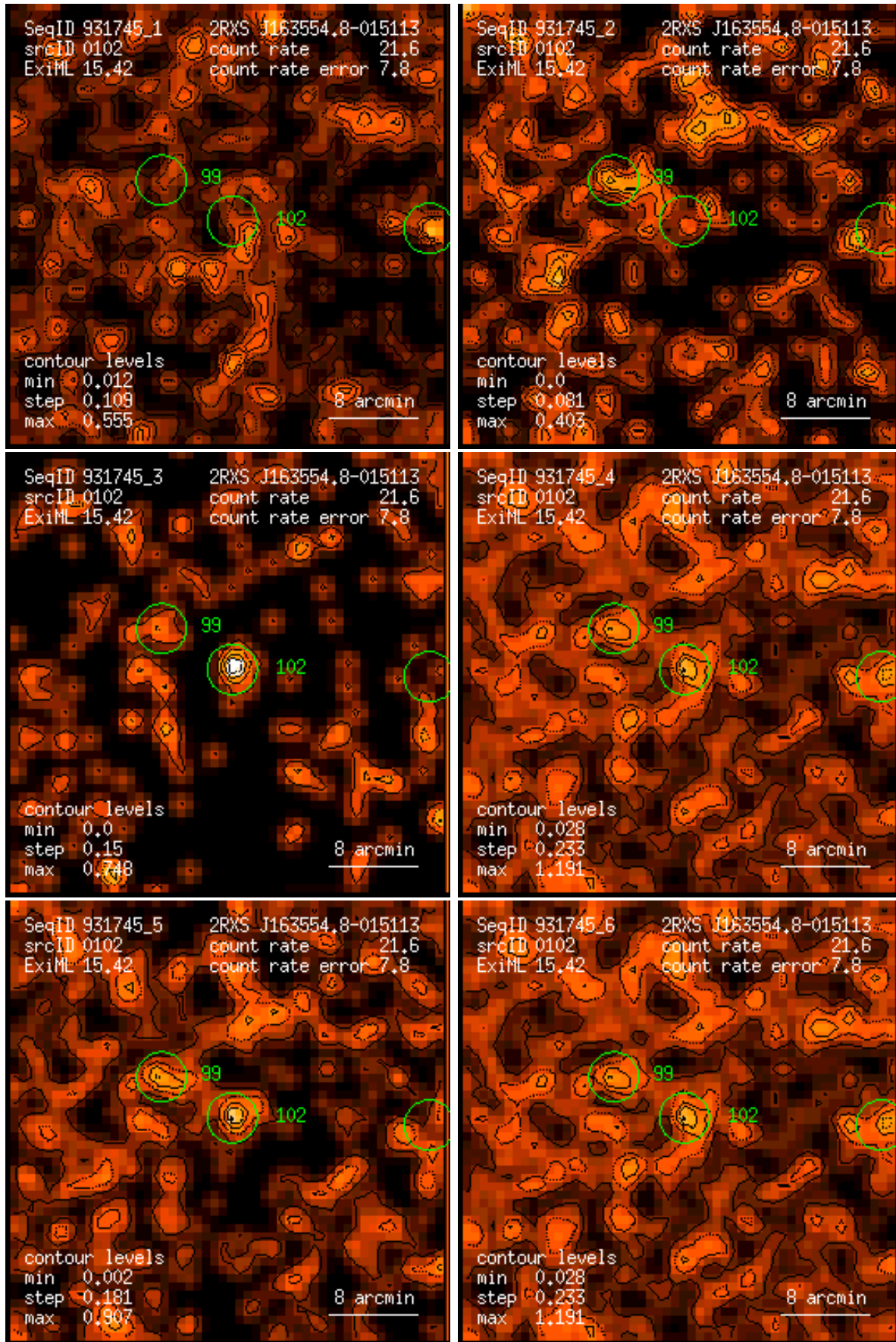
Figure 102: RASS 931745: detection 0102: band rate images, Gaussian filter: (1) PSPC channels 11 – 41, (2) 52 – 90, (3) 91 – 201, (4) 11 – 235, (5) 52 – 201, (6) 11 – 201. Broad band rates in counts/ks. Band rate contour levels in counts/ks/arcmin 2 .
