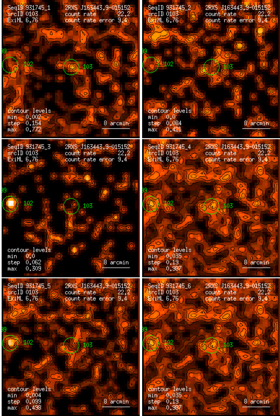
Figure 103: RASS 931745: detection 0103: band rate images, Gaussian filter: (1) PSPC channels 11 – 41, (2) 52 – 90, (3) 91 – 201, (4) 11 – 235, (5) 52 – 201, (6) 11 – 201. Broad band rates in counts/ks. Band rate contour levels in counts/ks/arcmin 2 .
