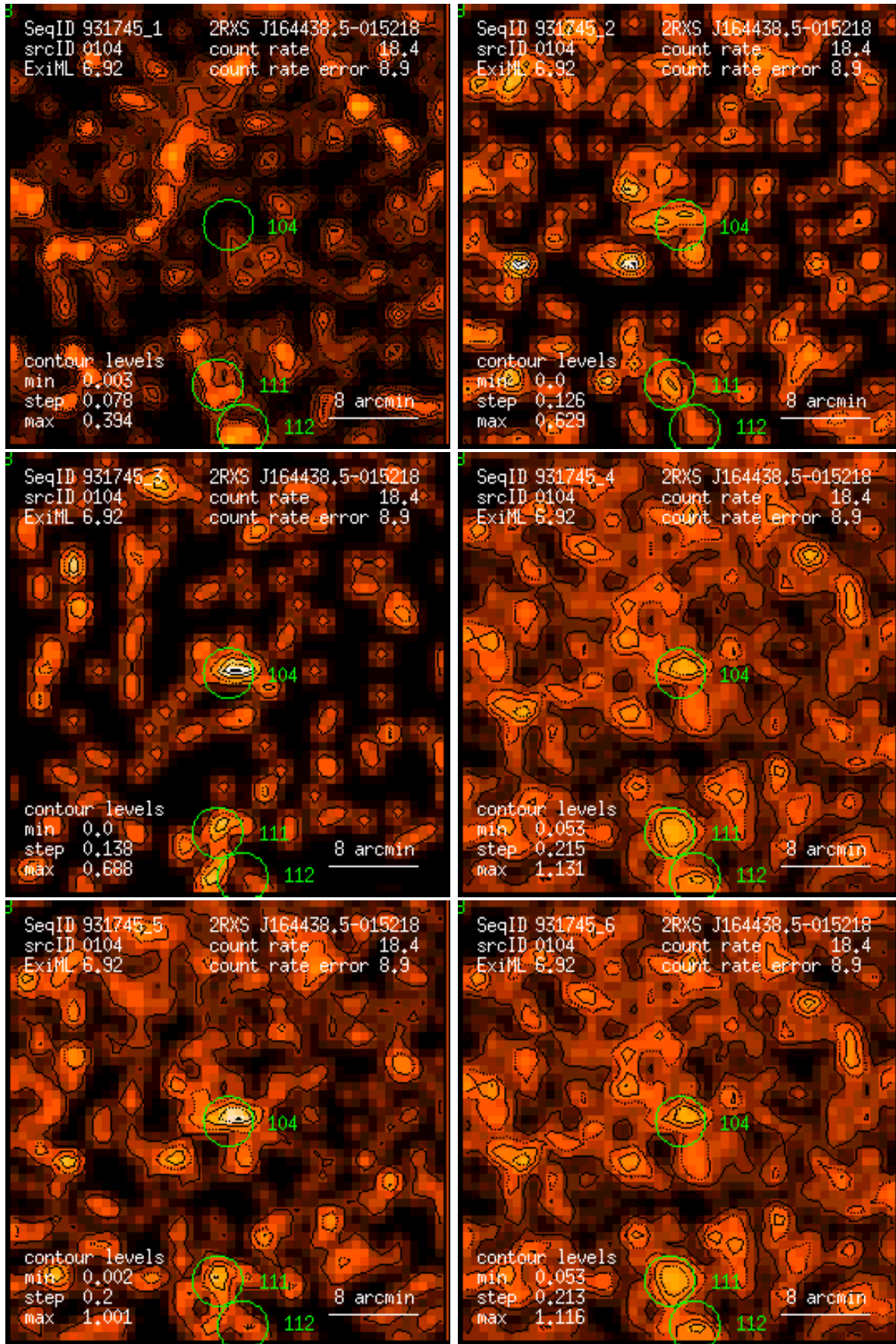
Figure 104: RASS 931745: detection 0104: band rate images, Gaussian filter: (1) PSPC channels 11 – 41, (2) 52 – 90, (3) 91 – 201, (4) 11 – 235, (5) 52 – 201, (6) 11 – 201. Broad band rates in counts/ks. Band rate contour levels in counts/ks/arcmin 2 .
