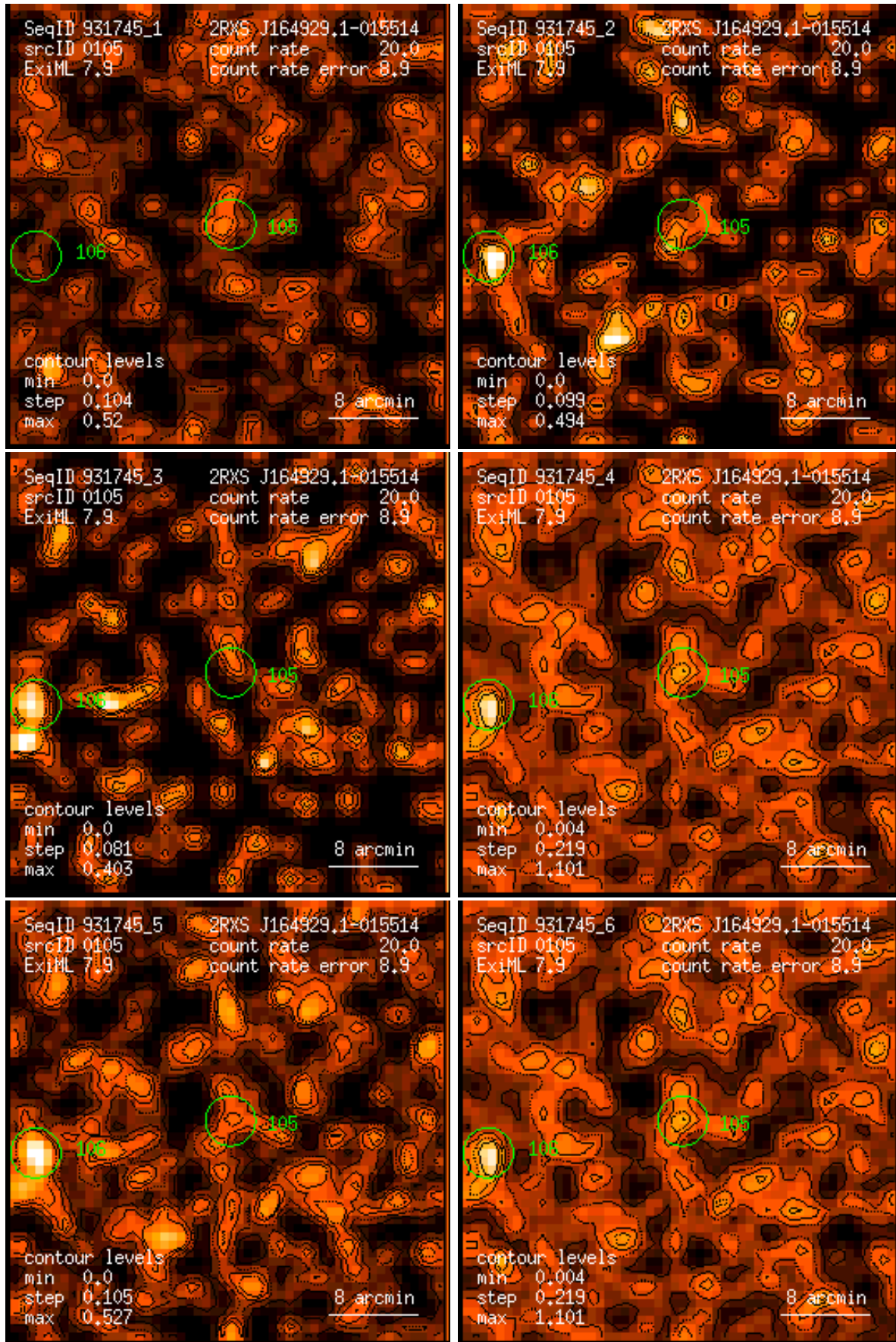
Figure 105: RASS 931745: detection 0105: band rate images, Gaussian filter: (1) PSPC channels 11 – 41, (2) 52 – 90, (3) 91 – 201, (4) 11 – 235, (5) 52 – 201, (6) 11 – 201. Broad band rates in counts/ks. Band rate contour levels in counts/ks/arcmin 2 .
