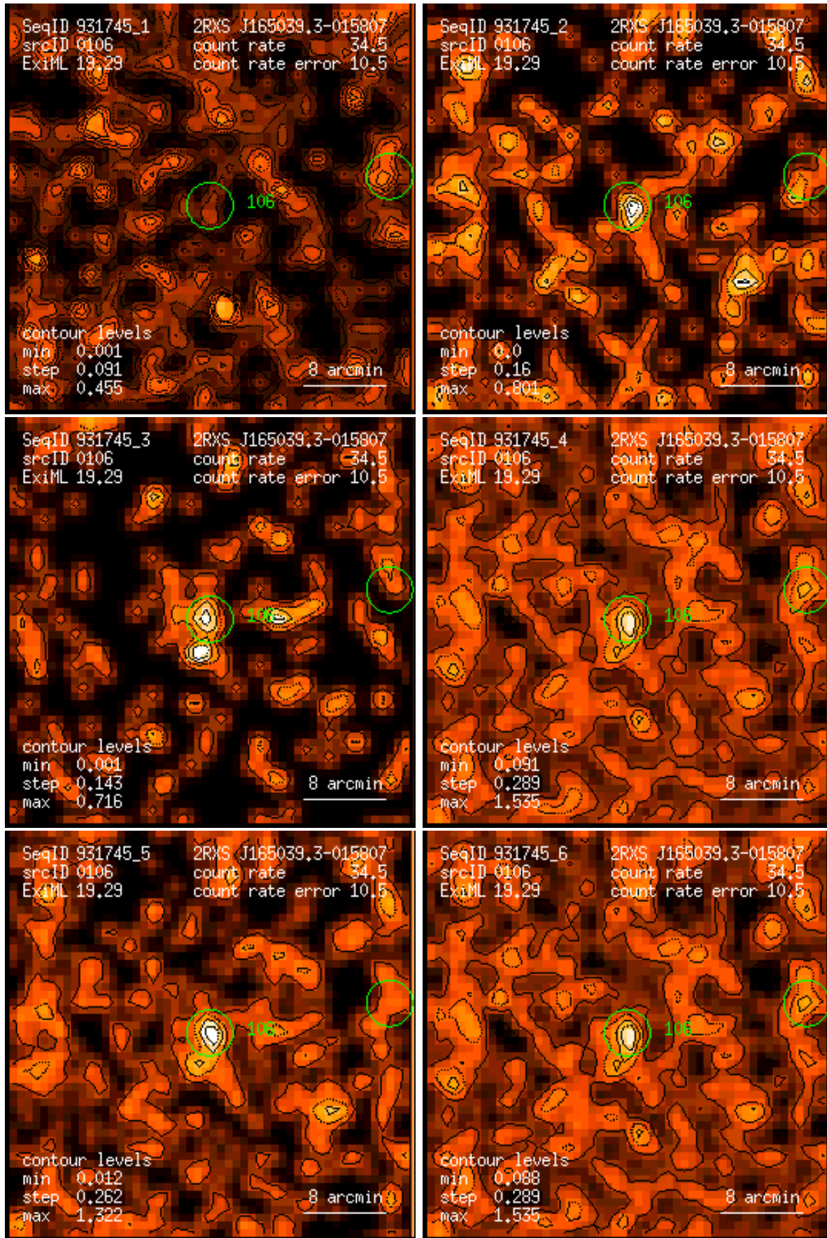
Figure 106: RASS 931745: detection 0106: band rate images, Gaussian filter: (1) PSPC channels 11 – 41, (2) 52 – 90, (3) 91 – 201, (4) 11 – 235, (5) 52 – 201, (6) 11 – 201. Broad band rates in counts/ks. Band rate contour levels in counts/ks/arcmin 2 .
