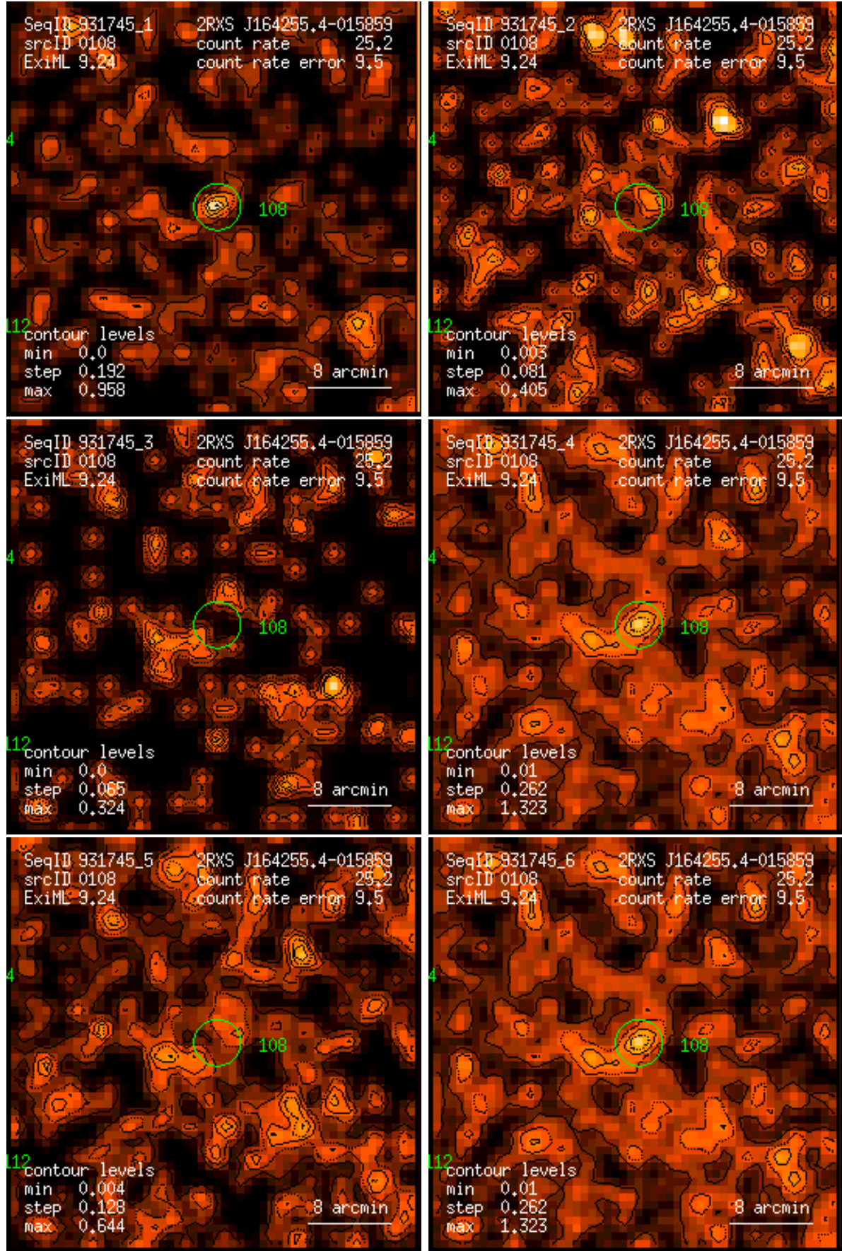
Figure 108: RASS 931745: detection 0108: band rate images, Gaussian filter: (1) PSPC channels 11 – 41, (2) 52 – 90, (3) 91 – 201, (4) 11 – 235, (5) 52 – 201, (6) 11 – 201. Broad band rates in counts/ks. Band rate contour levels in counts/ks/arcmin 2 .
