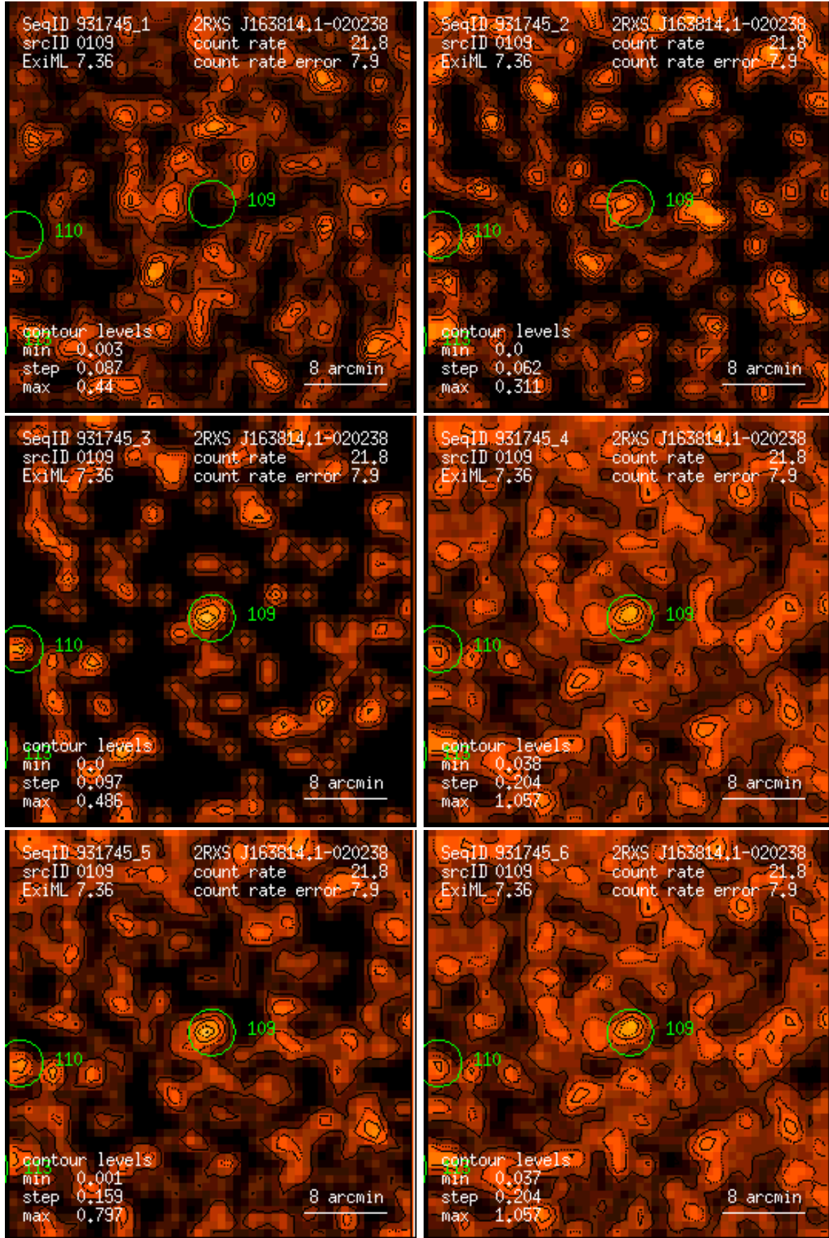
Figure 109: RASS 931745: detection 0109: band rate images, Gaussian filter: (1) PSPC channels 11 – 41, (2) 52 – 90, (3) 91 – 201, (4) 11 – 235, (5) 52 – 201, (6) 11 – 201. Broad band rates in counts/ks. Band rate contour levels in counts/ks/arcmin 2 .
