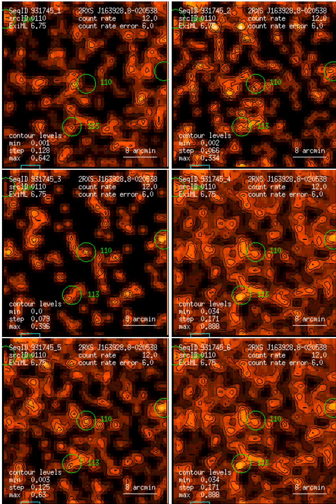
Figure 110: RASS 931745: detection 0110: band rate images, Gaussian filter: (1) PSPC channels 11 – 41, (2) 52 – 90, (3) 91 – 201, (4) 11 – 235, (5) 52 – 201, (6) 11 – 201. Broad band rates in counts/ks. Band rate contour levels in counts/ks/arcmin 2 .
