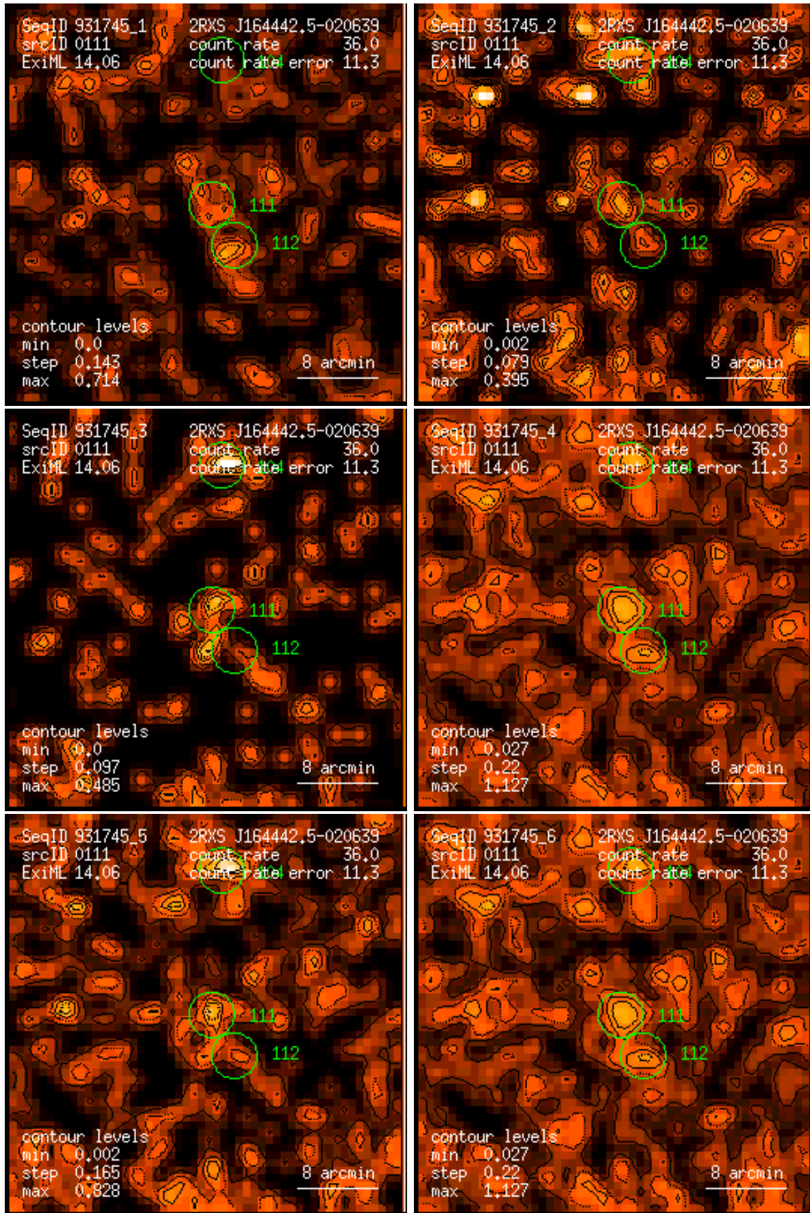
Figure 111: RASS 931745: detection 0111: band rate images, Gaussian filter: (1) PSPC channels 11 – 41, (2) 52 – 90, (3) 91 – 201, (4) 11 – 235, (5) 52 – 201, (6) 11 – 201. Broad band rates in counts/ks. Band rate contour levels in counts/ks/arcmin 2 .
