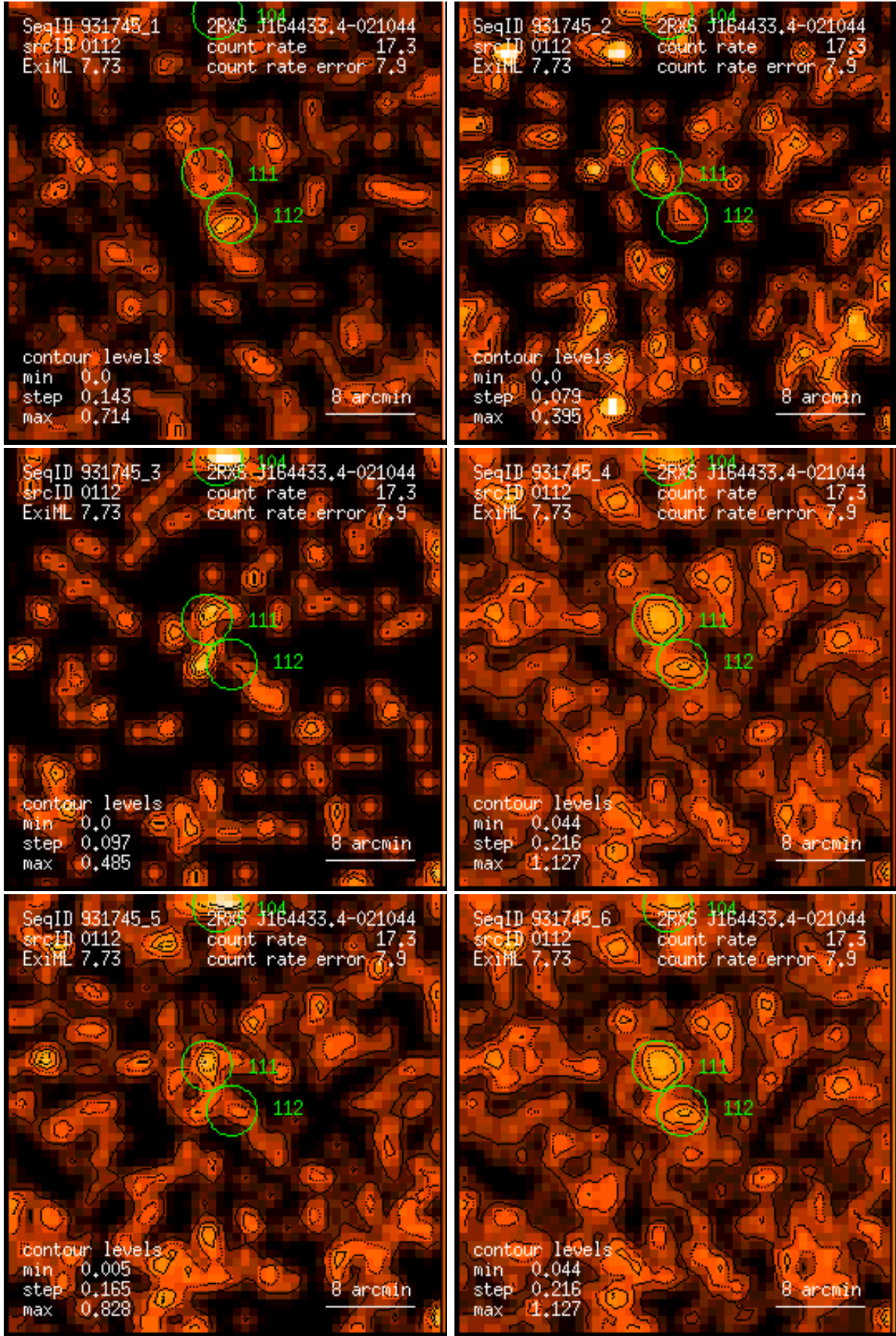
Figure 112: RASS 931745: detection 0112: band rate images, Gaussian filter: (1) PSPC channels 11 – 41, (2) 52 – 90, (3) 91 – 201, (4) 11 – 235, (5) 52 – 201, (6) 11 – 201. Broad band rates in counts/ks. Band rate contour levels in counts/ks/arcmin 2 .
