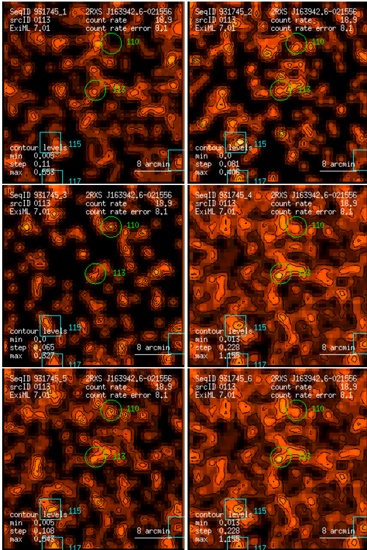
Figure 113: RASS 931745: detection 0113: band rate images, Gaussian filter: (1) PSPC channels 11 – 41, (2) 52 – 90, (3) 91 – 201, (4) 11 – 235, (5) 52 – 201, (6) 11 – 201. Broad band rates in counts/ks. Band rate contour levels in counts/ks/arcmin 2 .
