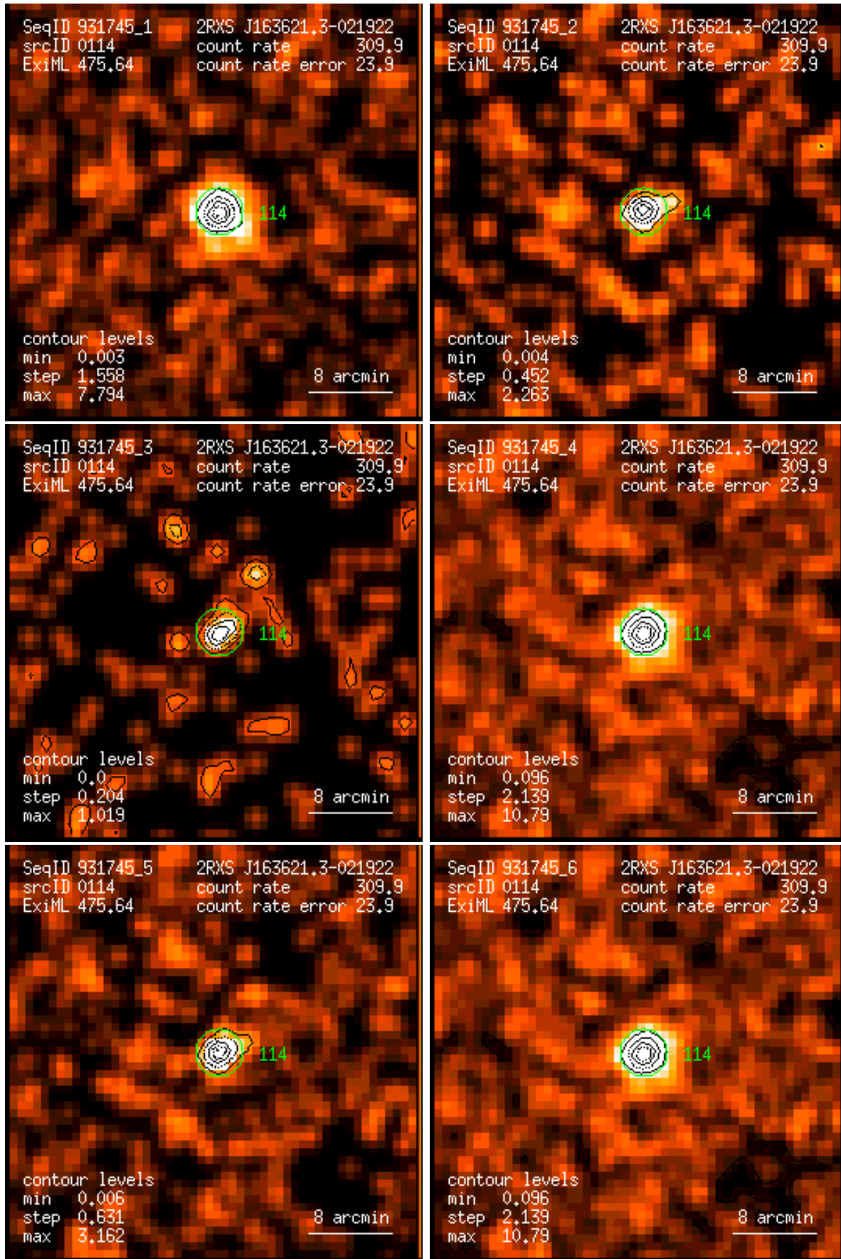
Figure 114: RASS 931745: detection 0114: band rate images, Gaussian filter: (1) PSPC channels 11 – 41, (2) 52 – 90, (3) 91 – 201, (4) 11 – 235, (5) 52 – 201, (6) 11 – 201. Broad band rates in counts/ks. Band rate contour levels in counts/ks/arcmin 2 .
