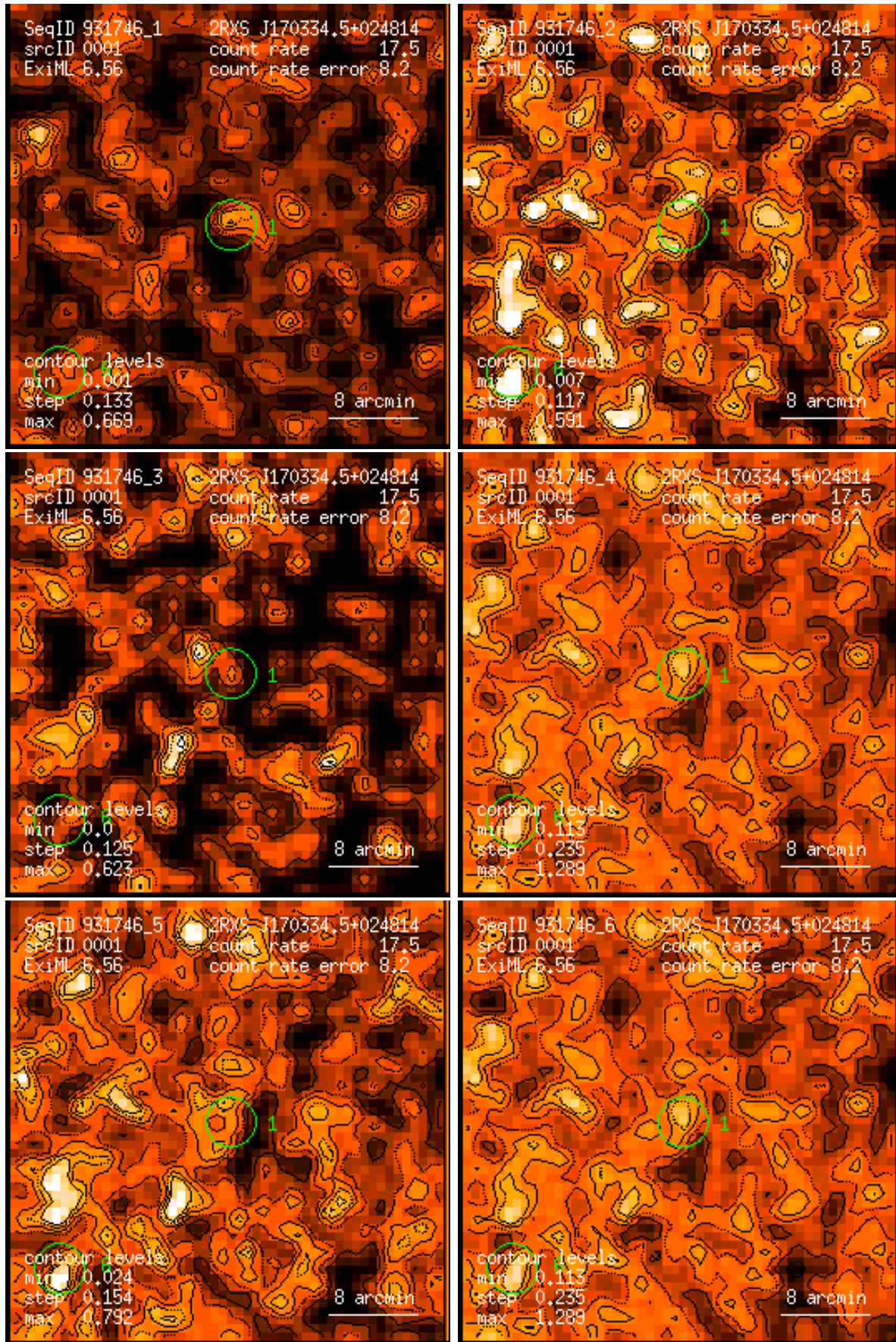
Figure 1: RASS 931746: detection 0001: band rate images, Gaussian filter: (1) PSPC channels 11 – 41, (2) 52 – 90, (3) 91 – 201, (4) 11 – 235, (5) 52 – 201, (6) 11 – 201. Broad band rates in counts/ks. Band rate contour levels in counts/ks/arcmin 2 .
