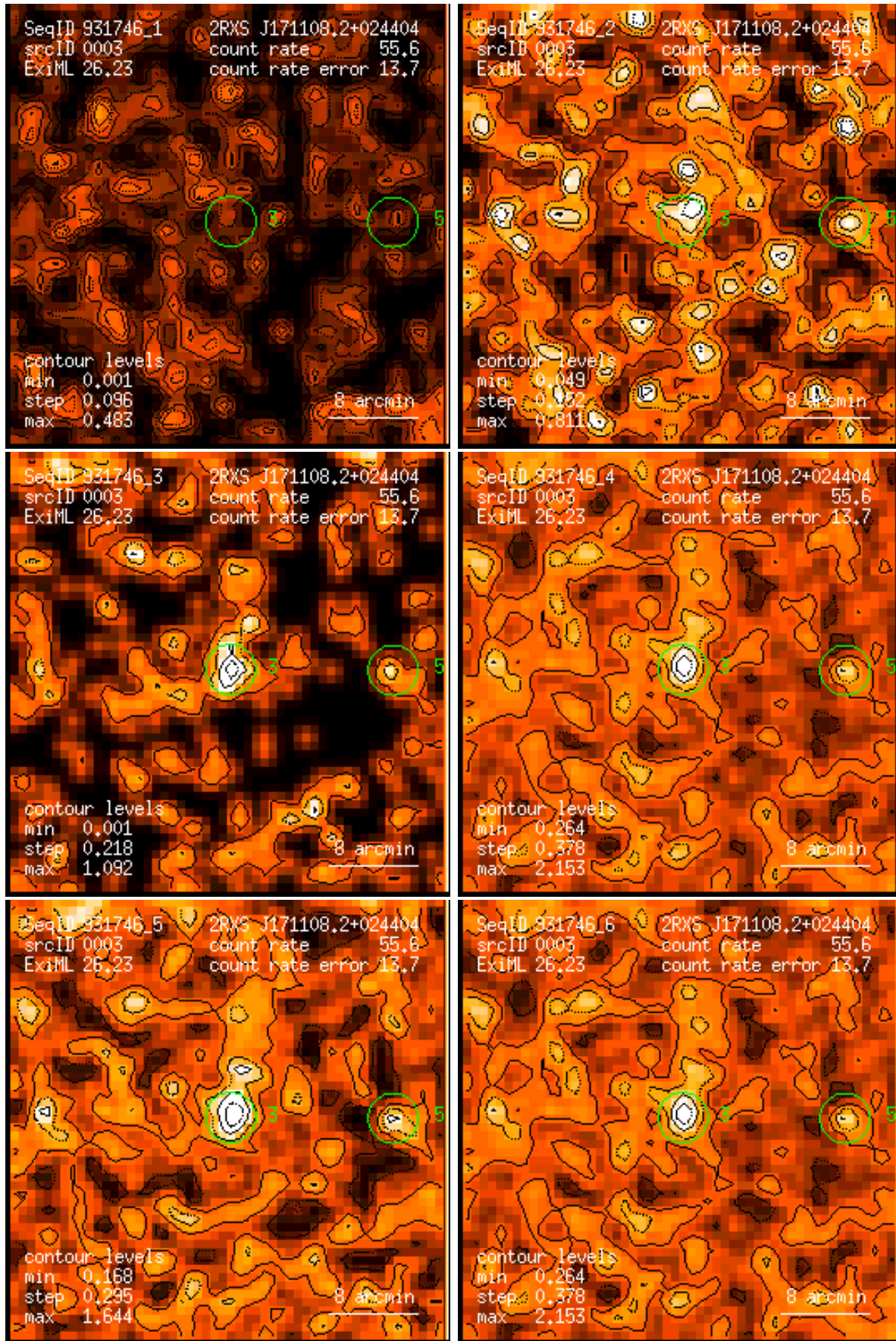
Figure 3: RASS 931746: detection 0003: band rate images, Gaussian filter: (1) PSPC channels 11 – 41, (2) 52 – 90, (3) 91 – 201, (4) 11 – 235, (5) 52 – 201, (6) 11 – 201. Broad band rates in counts/ks. Band rate contour levels in counts/ks/arcmin 2 .
