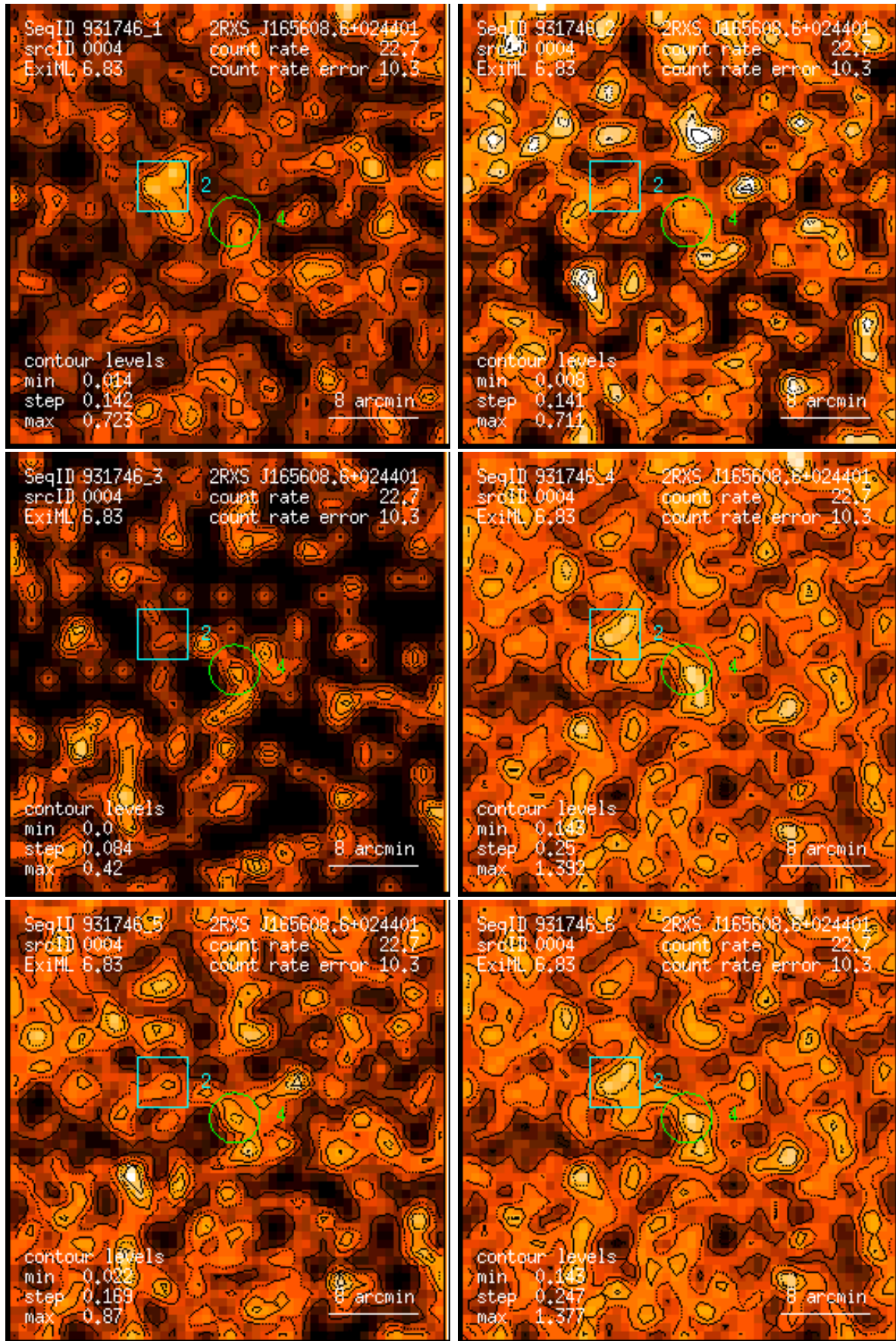
Figure 4: RASS 931746: detection 0004: band rate images, Gaussian filter: (1) PSPC channels 11 – 41, (2) 52 – 90, (3) 91 – 201, (4) 11 – 235, (5) 52 – 201, (6) 11 – 201. Broad band rates in counts/ks. Band rate contour levels in counts/ks/arcmin 2 .
