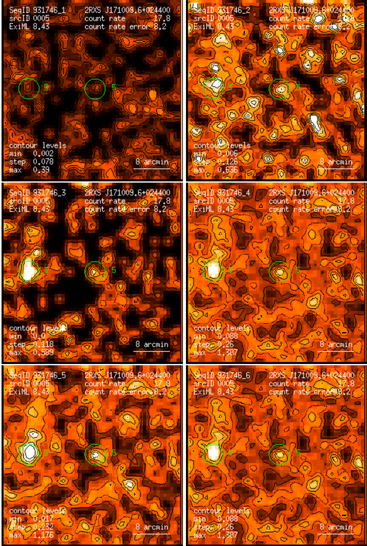
Figure 5: RASS 931746: detection 0005: band rate images, Gaussian filter: (1) PSPC channels 11 – 41, (2) 52 – 90, (3) 91 – 201, (4) 11 – 235, (5) 52 – 201, (6) 11 – 201. Broad band rates in counts/ks. Band rate contour levels in counts/ks/arcmin 2 .
