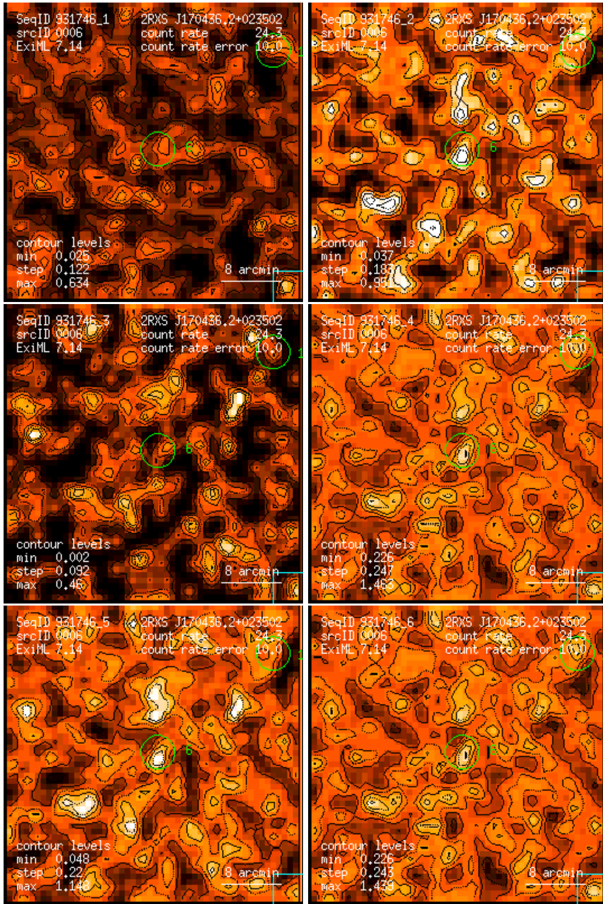
Figure 6: RASS 931746: detection 0006: band rate images, Gaussian filter: (1) PSPC channels 11 – 41, (2) 52 – 90, (3) 91 – 201, (4) 11 – 235, (5) 52 – 201, (6) 11 – 201. Broad band rates in counts/ks. Band rate contour levels in counts/ks/arcmin 2 .
