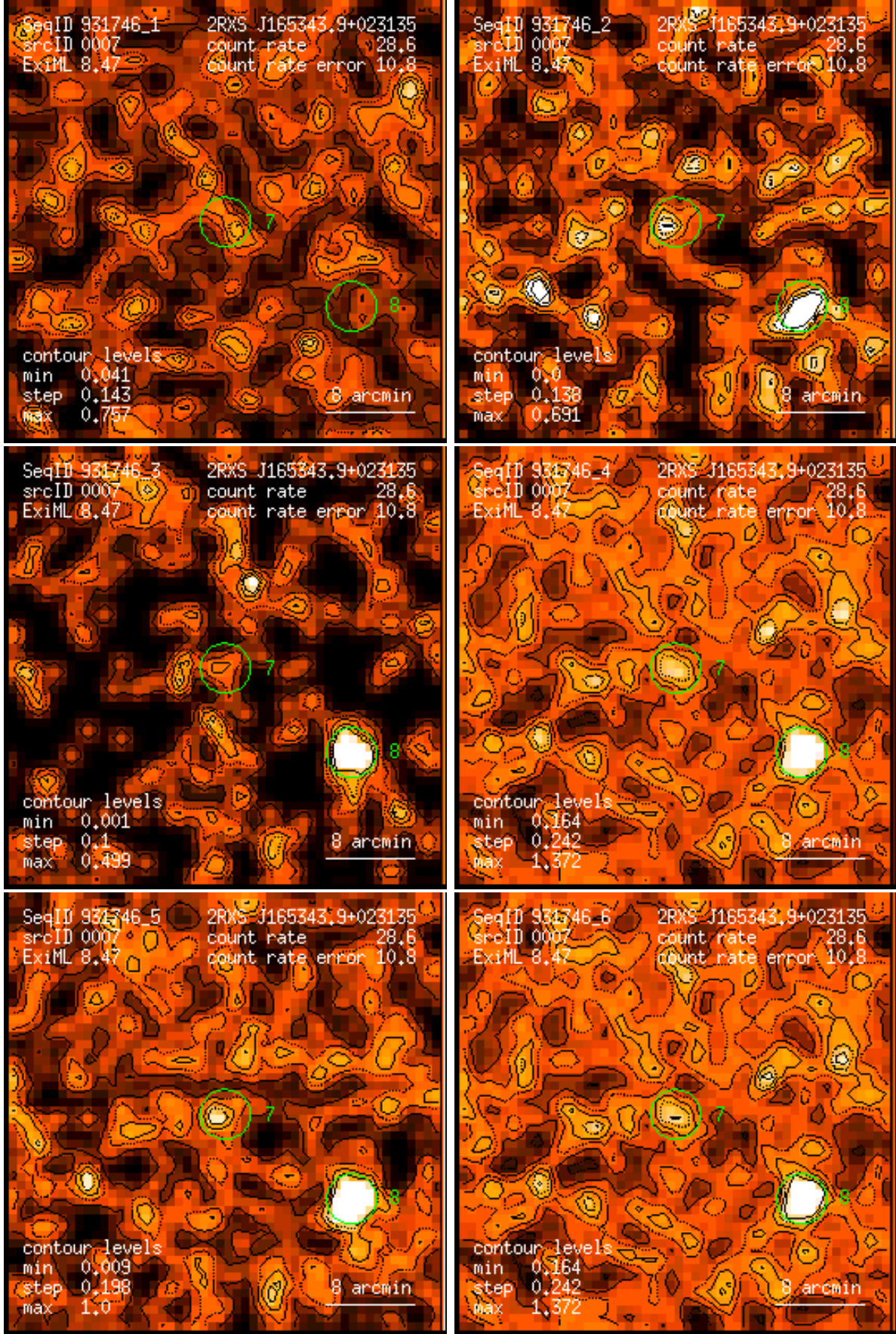
Figure 7: RASS 931746: detection 0007: band rate images, Gaussian filter: (1) PSPC channels 11 – 41, (2) 52 – 90, (3) 91 – 201, (4) 11 – 235, (5) 52 – 201, (6) 11 – 201. Broad band rates in counts/ks. Band rate contour levels in counts/ks/arcmin 2 .
