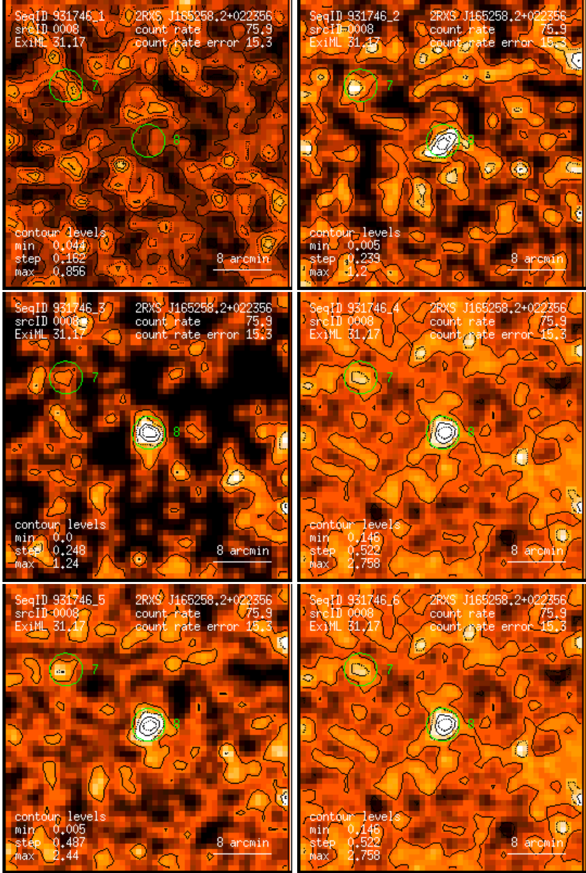
Figure 8: RASS 931746: detection 0008: band rate images, Gaussian filter: (1) PSPC channels 11 – 41, (2) 52 – 90, (3) 91 – 201, (4) 11 – 235, (5) 52 – 201, (6) 11 – 201. Broad band rates in counts/ks. Band rate contour levels in counts/ks/arcmin 2 .
