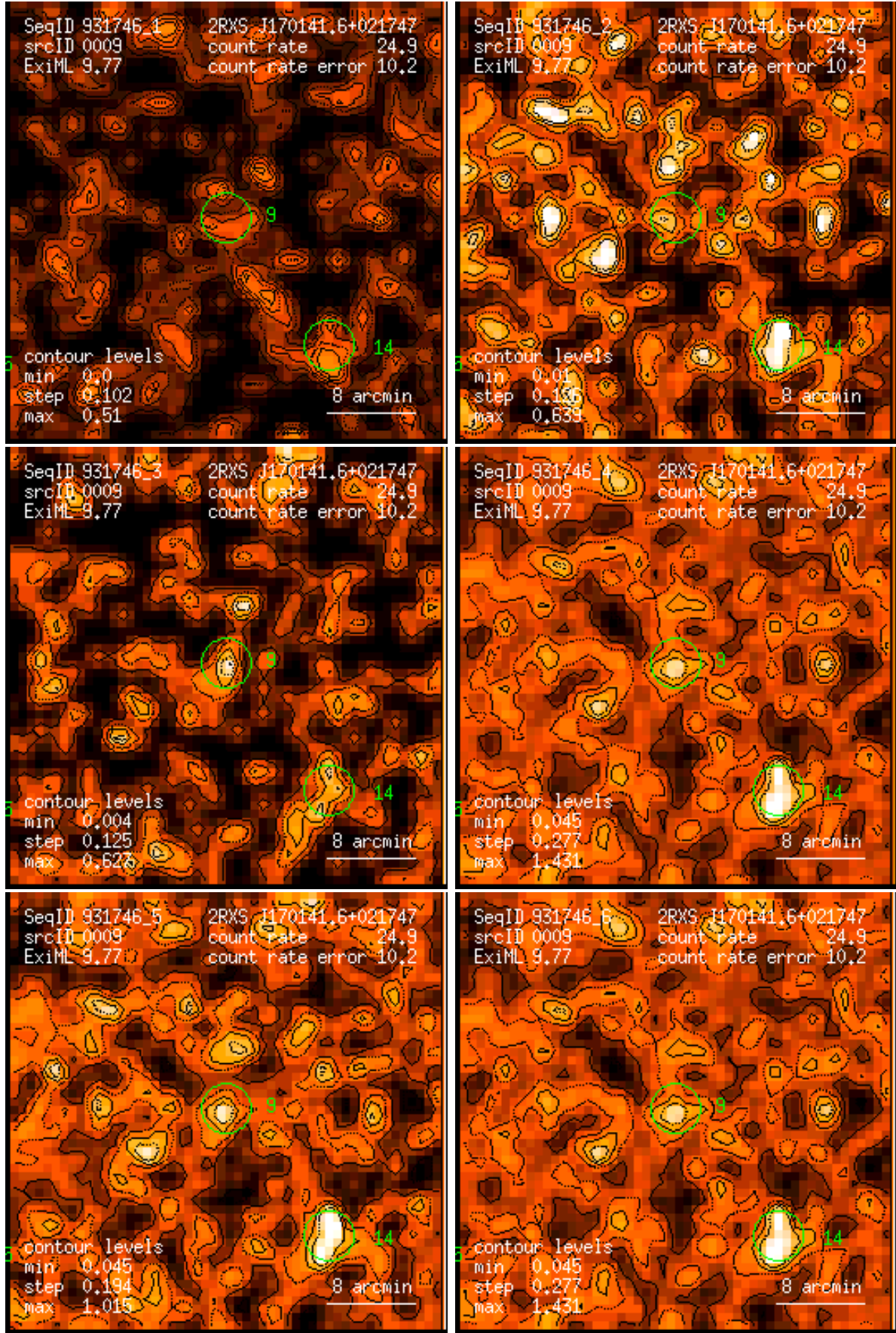
Figure 9: RASS 931746: detection 0009: band rate images, Gaussian filter: (1) PSPC channels 11 – 41, (2) 52 – 90, (3) 91 – 201, (4) 11 – 235, (5) 52 – 201, (6) 11 – 201. Broad band rates in counts/ks. Band rate contour levels in counts/ks/arcmin 2 .
