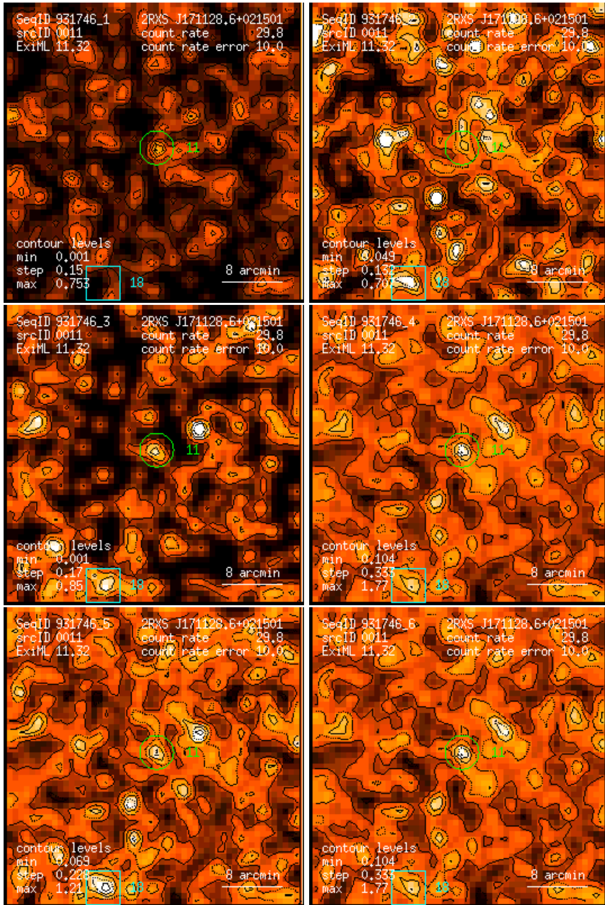
Figure 11: RASS 931746: detection 0011: band rate images, Gaussian filter: (1) PSPC channels 11 – 41, (2) 52 – 90, (3) 91 – 201, (4) 11 – 235, (5) 52 – 201, (6) 11 – 201. Broad band rates in counts/ks. Band rate contour levels in counts/ks/arcmin 2 .
