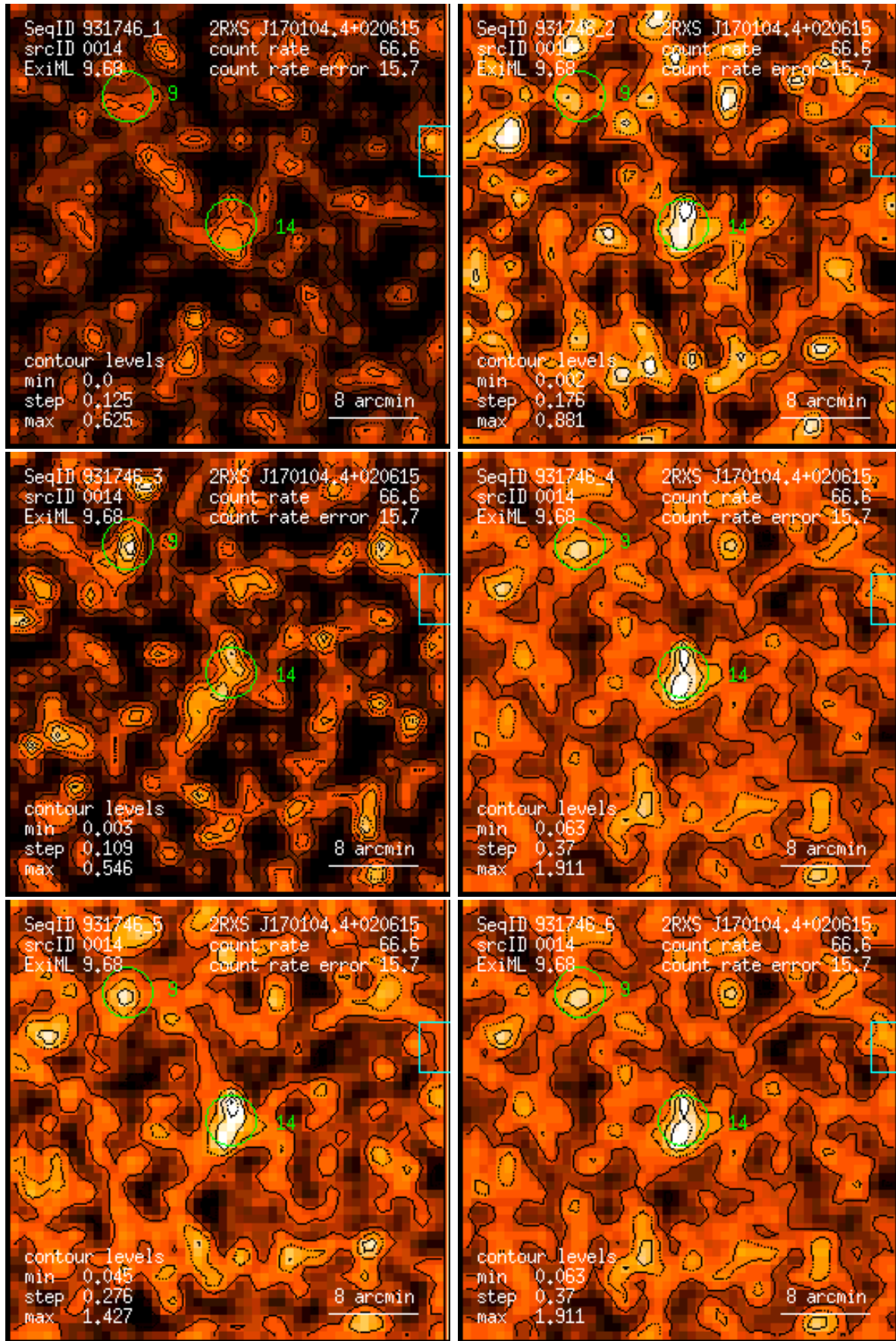
Figure 14: RASS 931746: detection 0014: band rate images, Gaussian filter: (1) PSPC channels 11 – 41, (2) 52 – 90, (3) 91 – 201, (4) 11 – 235, (5) 52 – 201, (6) 11 – 201. Broad band rates in counts/ks. Band rate contour levels in counts/ks/arcmin 2 .
