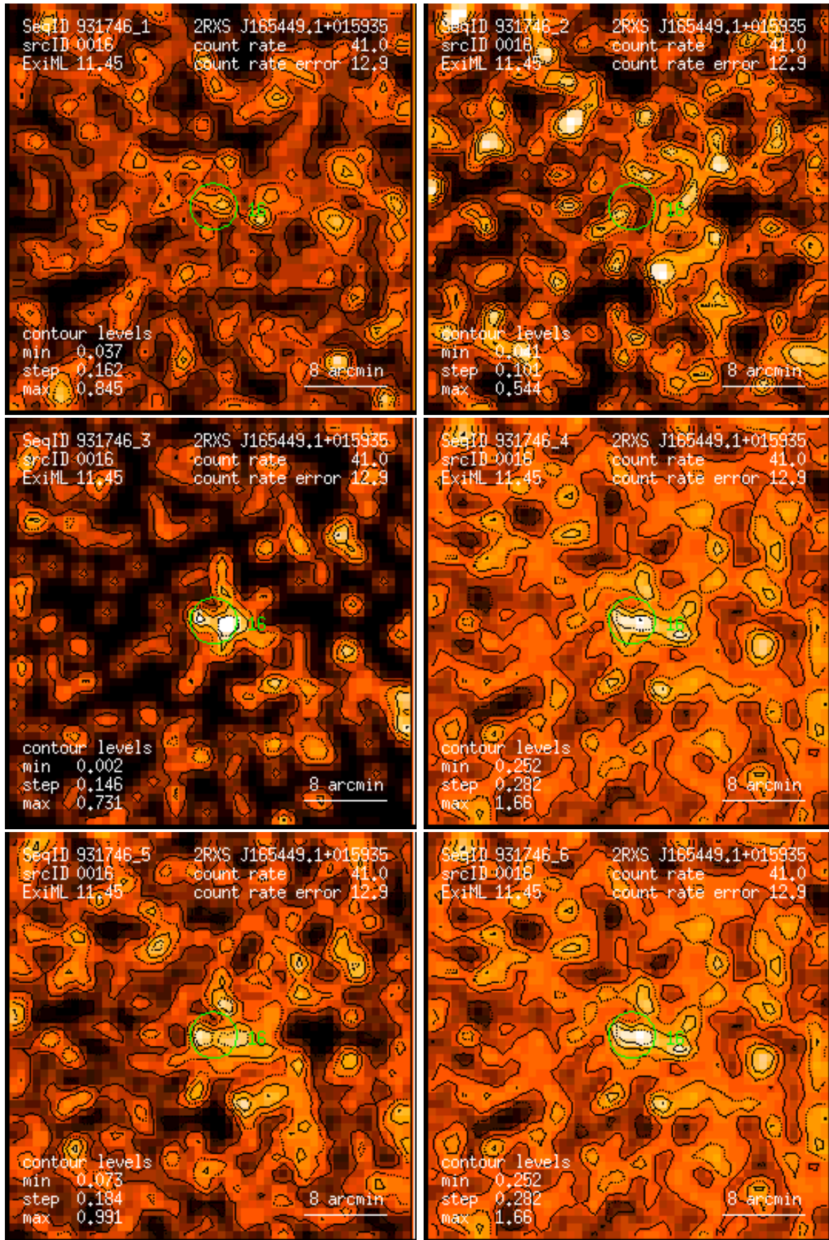
Figure 16: RASS 931746: detection 0016: band rate images, Gaussian filter: (1) PSPC channels 11 – 41, (2) 52 – 90, (3) 91 – 201, (4) 11 – 235, (5) 52 – 201, (6) 11 – 201. Broad band rates in counts/ks. Band rate contour levels in counts/ks/arcmin 2 .
