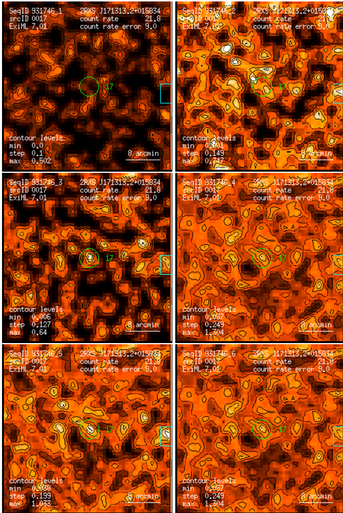
Figure 17: RASS 931746: detection 0017: band rate images, Gaussian filter: (1) PSPC channels 11 – 41, (2) 52 – 90, (3) 91 – 201, (4) 11 – 235, (5) 52 – 201, (6) 11 – 201. Broad band rates in counts/ks. Band rate contour levels in counts/ks/arcmin 2 .
