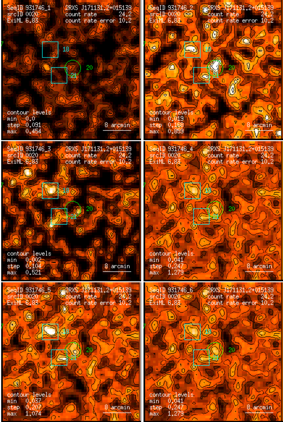
Figure 20: RASS 931746: detection 0020: band rate images, Gaussian filter: (1) PSPC channels 11 – 41, (2) 52 – 90, (3) 91 – 201, (4) 11 – 235, (5) 52 – 201, (6) 11 – 201. Broad band rates in counts/ks. Band rate contour levels in counts/ks/arcmin 2 .
