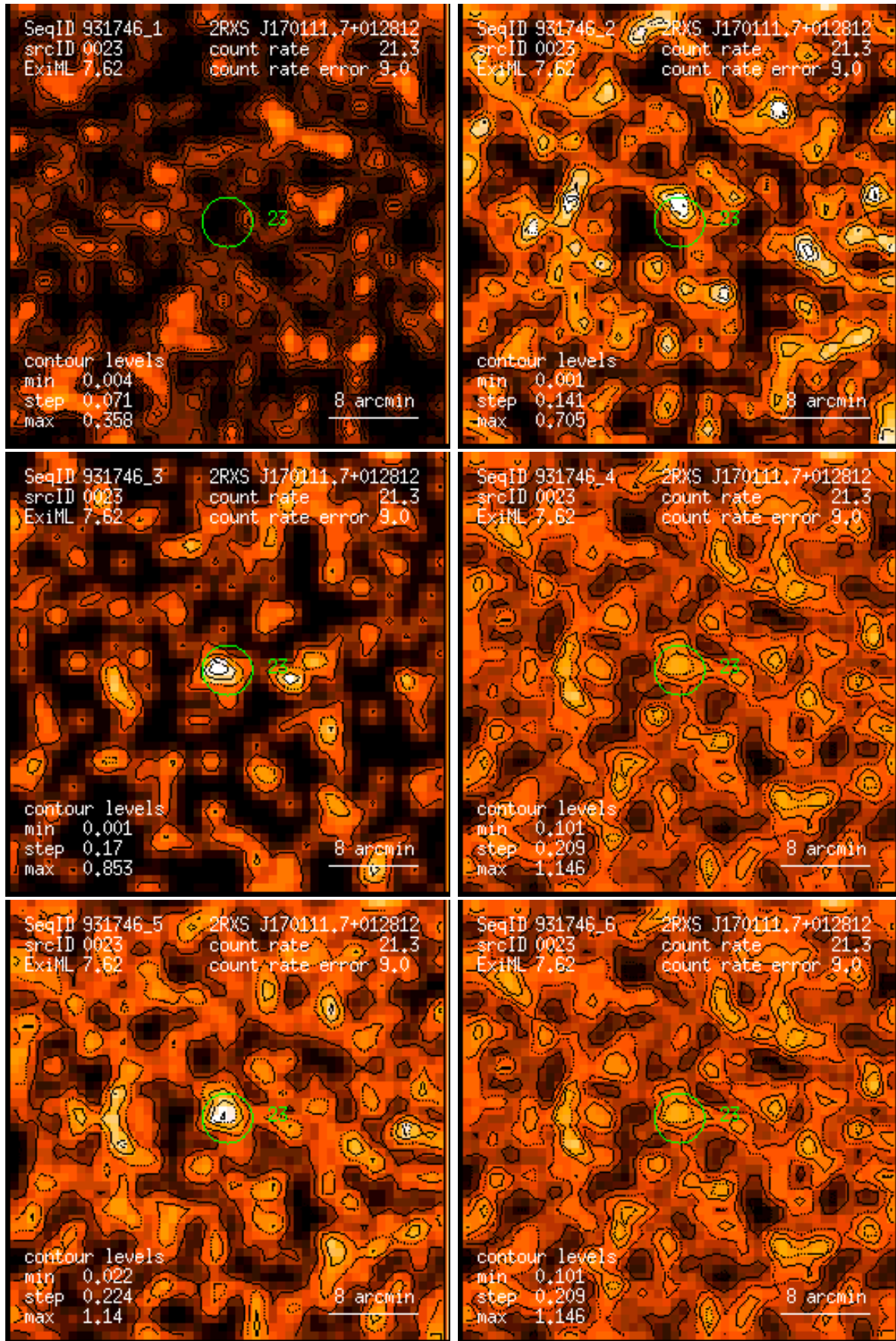
Figure 23: RASS 931746: detection 0023: band rate images, Gaussian filter: (1) PSPC channels 11 – 41, (2) 52 – 90, (3) 91 – 201, (4) 11 – 235, (5) 52 – 201, (6) 11 – 201. Broad band rates in counts/ks. Band rate contour levels in counts/ks/arcmin 2 .
