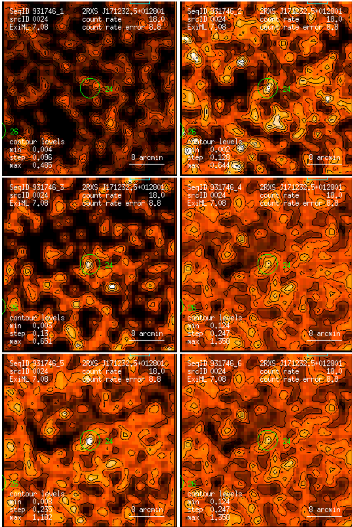
Figure 24: RASS 931746: detection 0024: band rate images, Gaussian filter: (1) PSPC channels 11 – 41, (2) 52 – 90, (3) 91 – 201, (4) 11 – 235, (5) 52 – 201, (6) 11 – 201. Broad band rates in counts/ks. Band rate contour levels in counts/ks/arcmin 2 .
