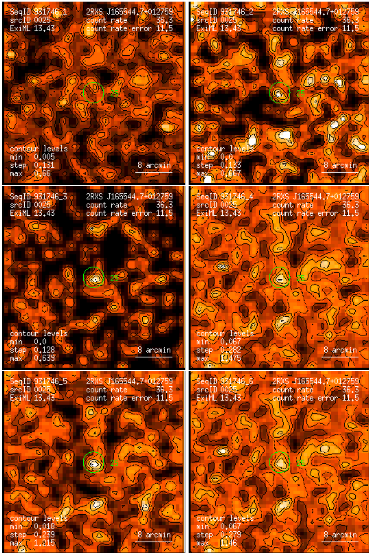
Figure 25: RASS 931746: detection 0025: band rate images, Gaussian filter: (1) PSPC channels 11 – 41, (2) 52 – 90, (3) 91 – 201, (4) 11 – 235, (5) 52 – 201, (6) 11 – 201. Broad band rates in counts/ks. Band rate contour levels in counts/ks/arcmin 2 .
