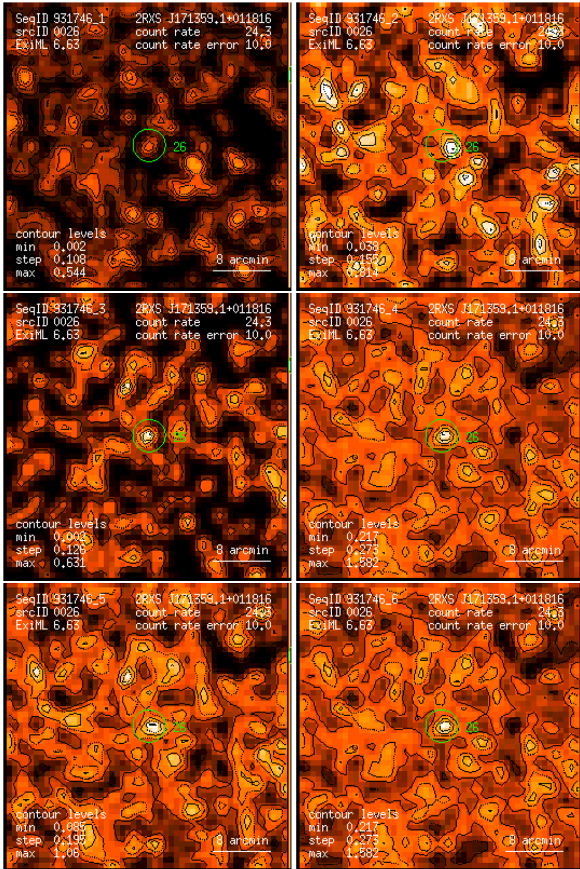
Figure 26: RASS 931746: detection 0026: band rate images, Gaussian filter: (1) PSPC channels 11 – 41, (2) 52 – 90, (3) 91 – 201, (4) 11 – 235, (5) 52 – 201, (6) 11 – 201. Broad band rates in counts/ks. Band rate contour levels in counts/ks/arcmin 2 .
