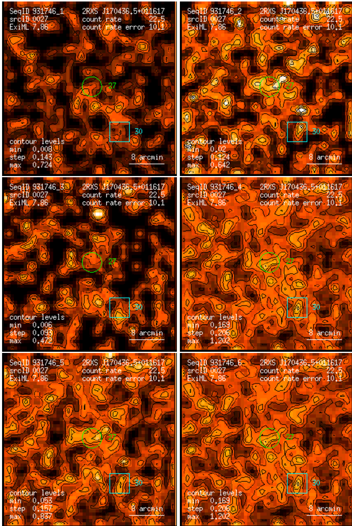
Figure 27: RASS 931746: detection 0027: band rate images, Gaussian filter: (1) PSPC channels 11 – 41, (2) 52 – 90, (3) 91 – 201, (4) 11 – 235, (5) 52 – 201, (6) 11 – 201. Broad band rates in counts/ks. Band rate contour levels in counts/ks/arcmin 2 .
