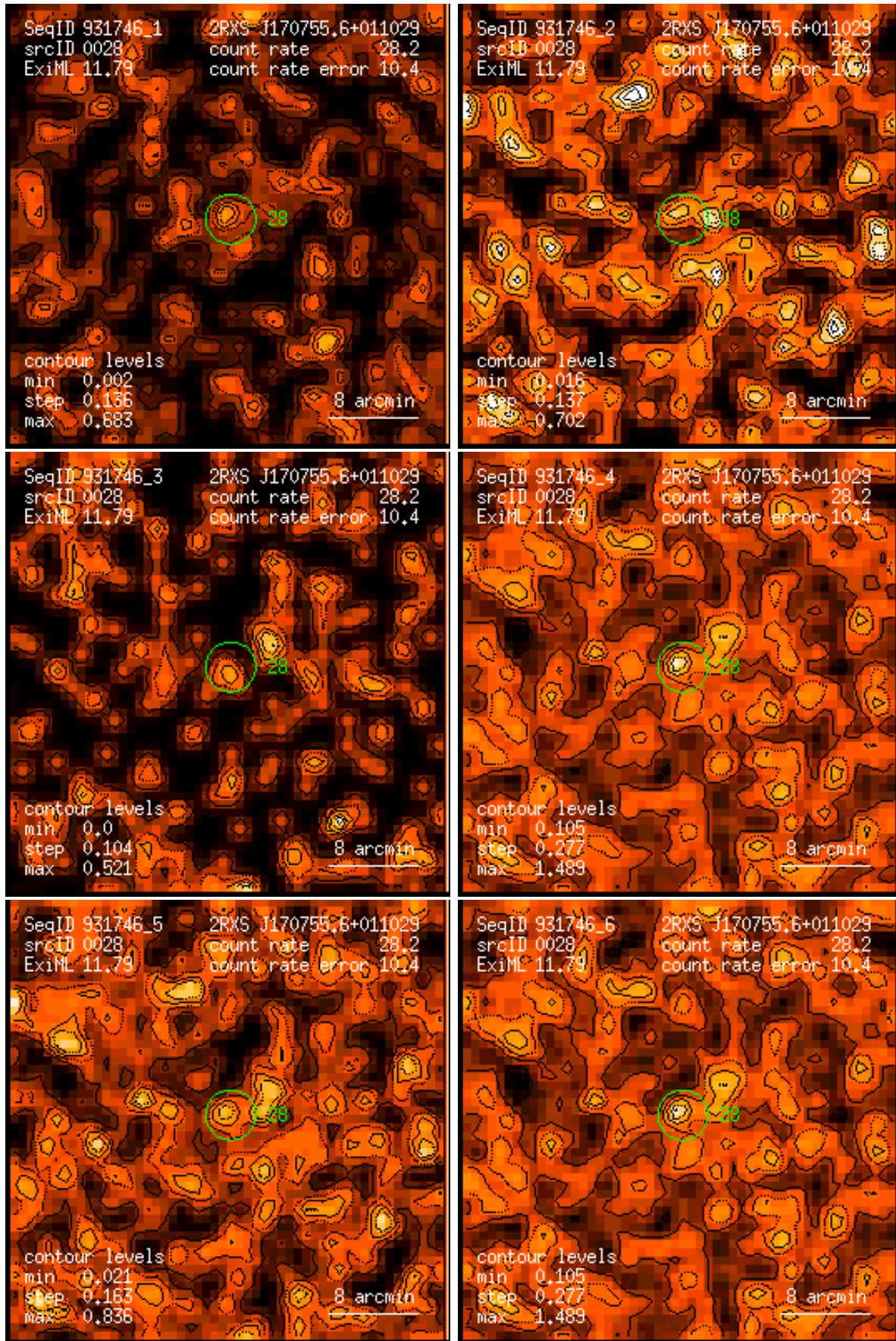
Figure 28: RASS 931746: detection 0028: band rate images, Gaussian filter: (1) PSPC channels 11 – 41, (2) 52 – 90, (3) 91 – 201, (4) 11 – 235, (5) 52 – 201, (6) 11 – 201. Broad band rates in counts/ks. Band rate contour levels in counts/ks/arcmin 2 .
