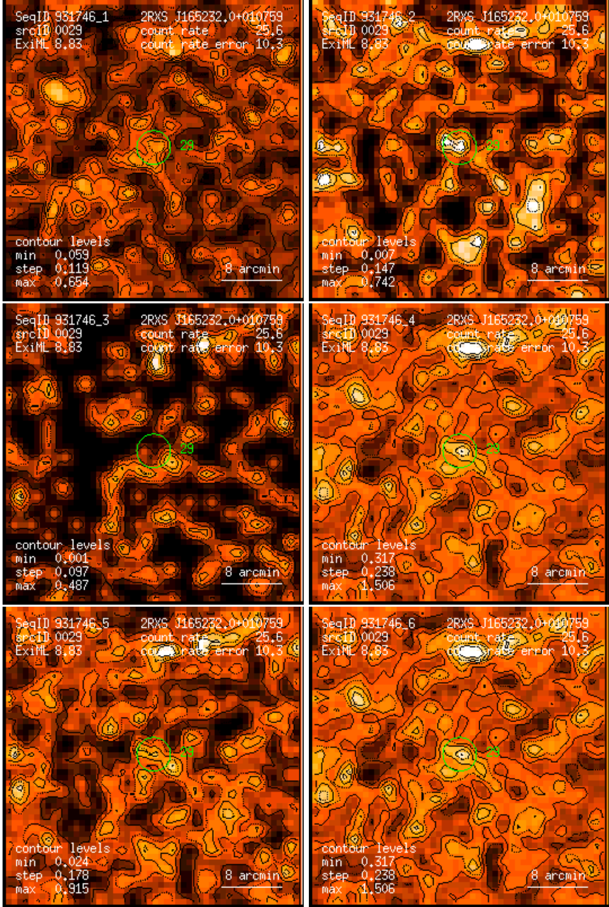
Figure 29: RASS 931746: detection 0029: band rate images, Gaussian filter: (1) PSPC channels 11 – 41, (2) 52 – 90, (3) 91 – 201, (4) 11 – 235, (5) 52 – 201, (6) 11 – 201. Broad band rates in counts/ks. Band rate contour levels in counts/ks/arcmin 2 .
