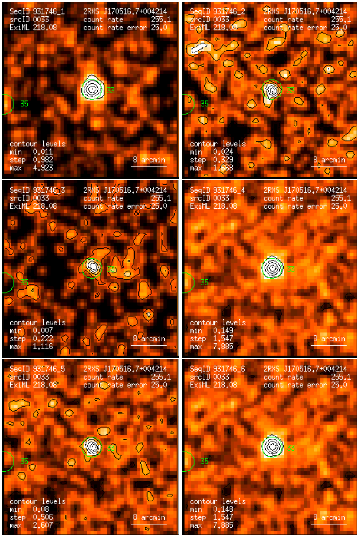
Figure 33: RASS 931746: detection 0033: band rate images, Gaussian filter: (1) PSPC channels 11 – 41, (2) 52 – 90, (3) 91 – 201, (4) 11 – 235, (5) 52 – 201, (6) 11 – 201. Broad band rates in counts/ks. Band rate contour levels in counts/ks/arcmin 2 .
