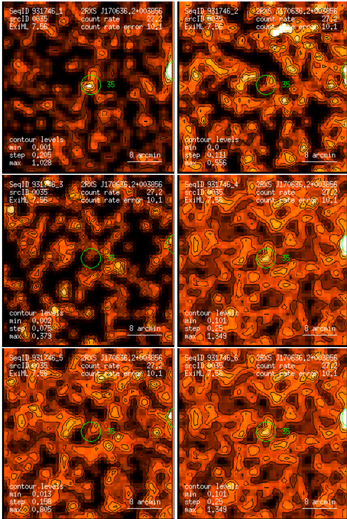
Figure 35: RASS 931746: detection 0035: band rate images, Gaussian filter: (1) PSPC channels 11 – 41, (2) 52 – 90, (3) 91 – 201, (4) 11 – 235, (5) 52 – 201, (6) 11 – 201. Broad band rates in counts/ks. Band rate contour levels in counts/ks/arcmin 2 .
