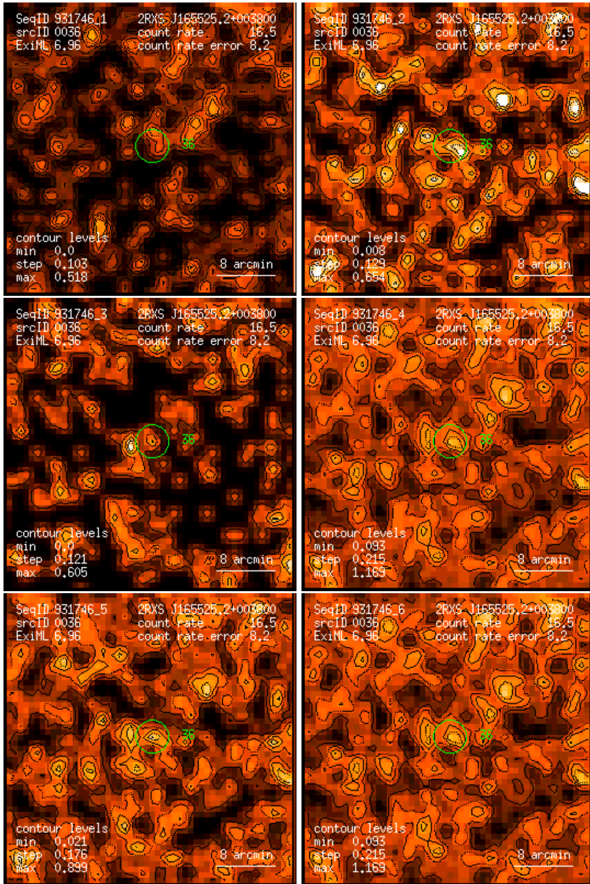
Figure 36: RASS 931746: detection 0036: band rate images, Gaussian filter: (1) PSPC channels 11 – 41, (2) 52 – 90, (3) 91 – 201, (4) 11 – 235, (5) 52 – 201, (6) 11 – 201. Broad band rates in counts/ks. Band rate contour levels in counts/ks/arcmin 2 .
