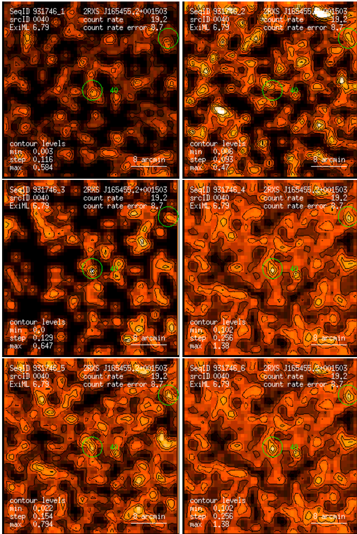
Figure 40: RASS 931746: detection 0040: band rate images, Gaussian filter: (1) PSPC channels 11 – 41, (2) 52 – 90, (3) 91 – 201, (4) 11 – 235, (5) 52 – 201, (6) 11 – 201. Broad band rates in counts/ks. Band rate contour levels in counts/ks/arcmin 2 .
