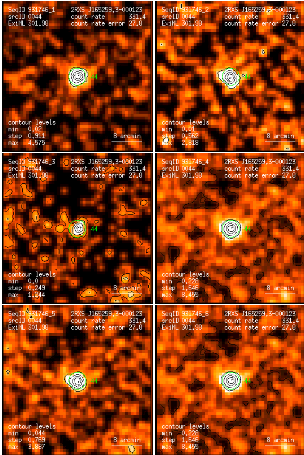
Figure 44: RASS 931746: detection 0044: band rate images, Gaussian filter: (1) PSPC channels 11 – 41, (2) 52 – 90, (3) 91 – 201, (4) 11 – 235, (5) 52 – 201, (6) 11 – 201. Broad band rates in counts/ks. Band rate contour levels in counts/ks/arcmin 2 .
