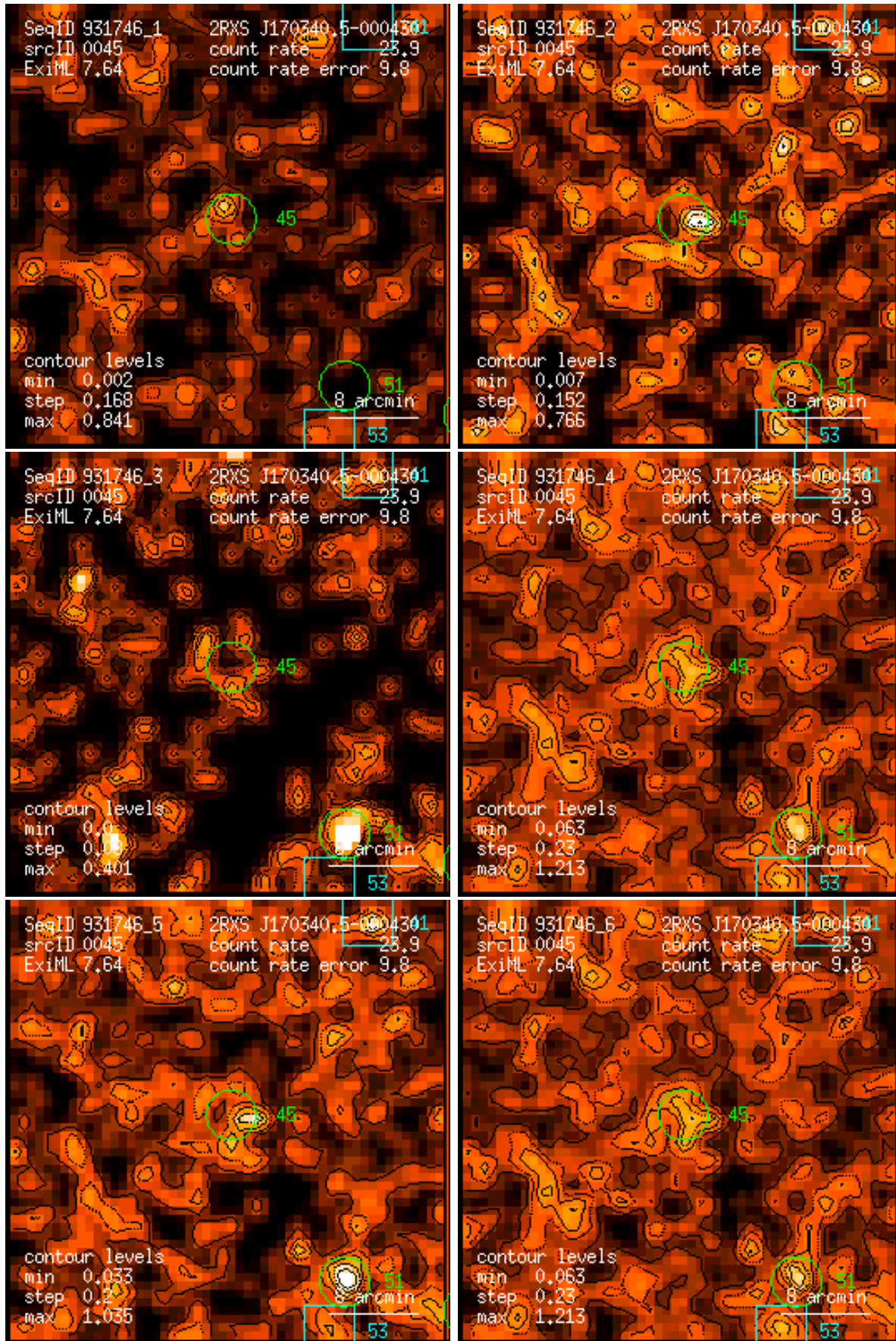
Figure 45: RASS 931746: detection 0045: band rate images, Gaussian filter: (1) PSPC channels 11 – 41, (2) 52 – 90, (3) 91 – 201, (4) 11 – 235, (5) 52 – 201, (6) 11 – 201. Broad band rates in counts/ks. Band rate contour levels in counts/ks/arcmin 2 .
