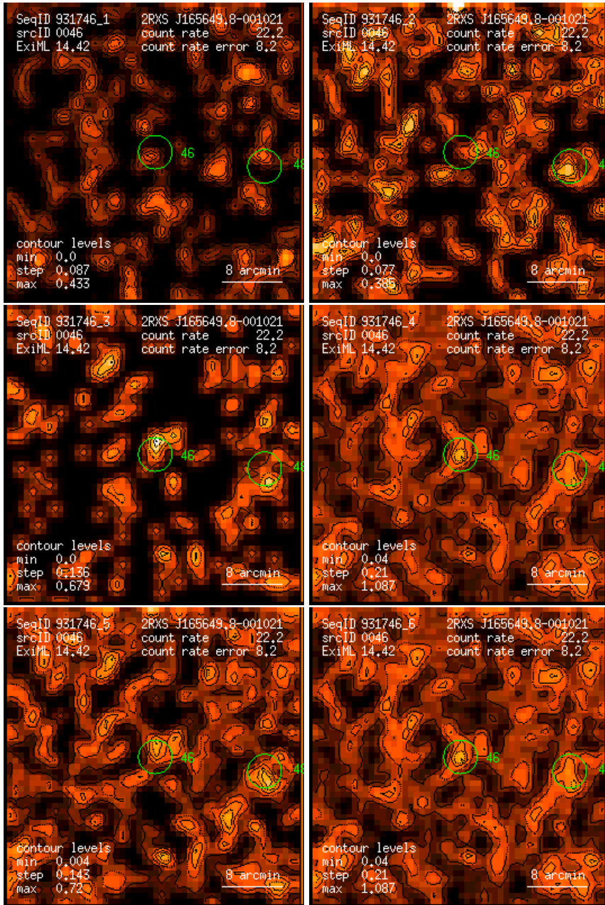
Figure 46: RASS 931746: detection 0046: band rate images, Gaussian filter: (1) PSPC channels 11 – 41, (2) 52 – 90, (3) 91 – 201, (4) 11 – 235, (5) 52 – 201, (6) 11 – 201. Broad band rates in counts/ks. Band rate contour levels in counts/ks/arcmin 2 .
