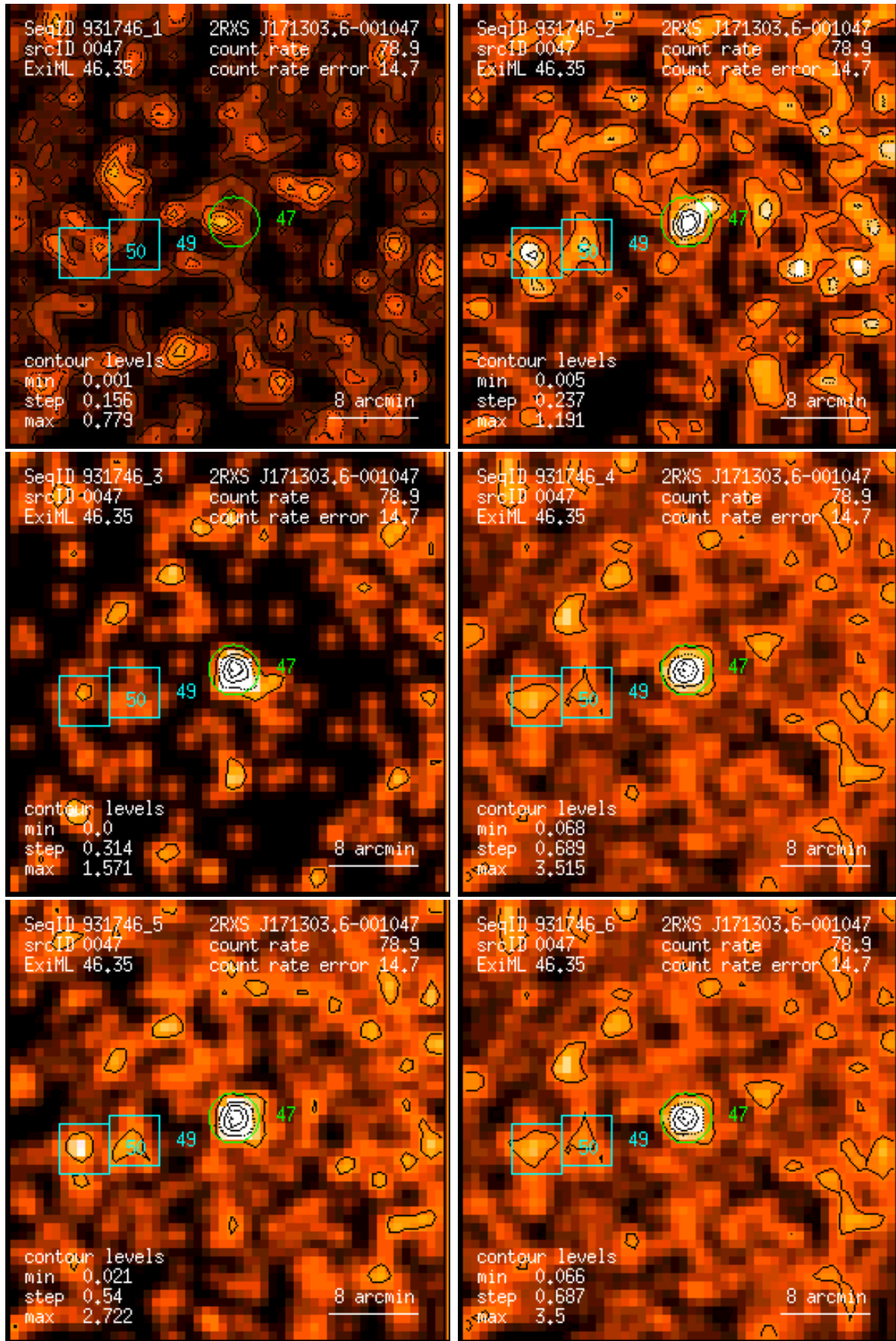
Figure 47: RASS 931746: detection 0047: band rate images, Gaussian filter: (1) PSPC channels 11 – 41, (2) 52 – 90, (3) 91 – 201, (4) 11 – 235, (5) 52 – 201, (6) 11 – 201. Broad band rates in counts/ks. Band rate contour levels in counts/ks/arcmin 2 .
