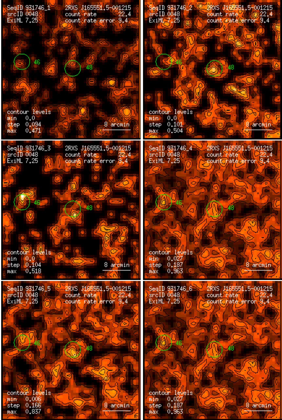
Figure 48: RASS 931746: detection 0048: band rate images, Gaussian filter: (1) PSPC channels 11 – 41, (2) 52 – 90, (3) 91 – 201, (4) 11 – 235, (5) 52 – 201, (6) 11 – 201. Broad band rates in counts/ks. Band rate contour levels in counts/ks/arcmin 2 .
